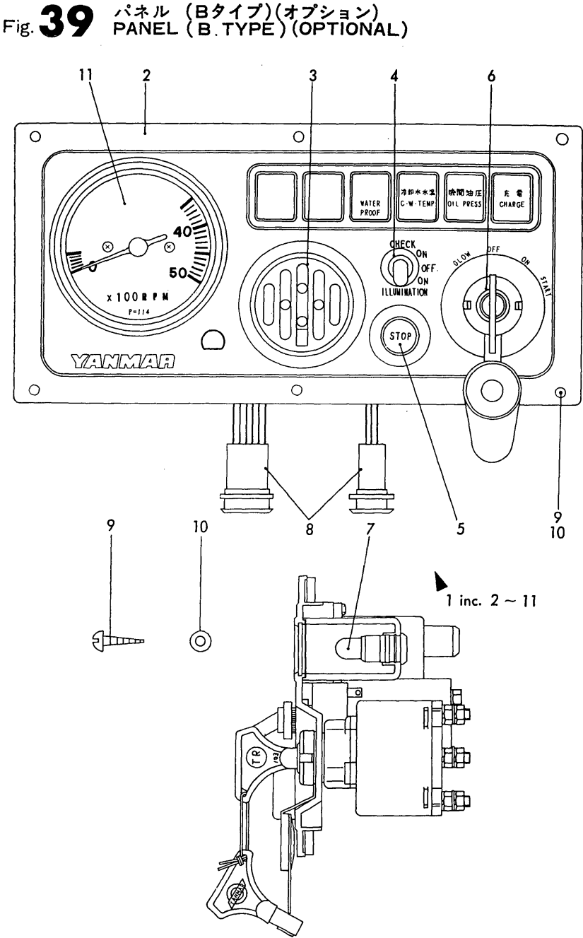
Fig.39.PANEL(B TYPE)(OPTIONAL)
