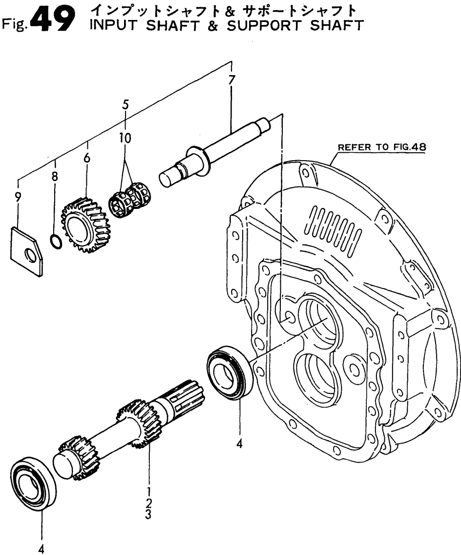
Fig.49.INPUT SHAFT & SURPORT SHAFT
