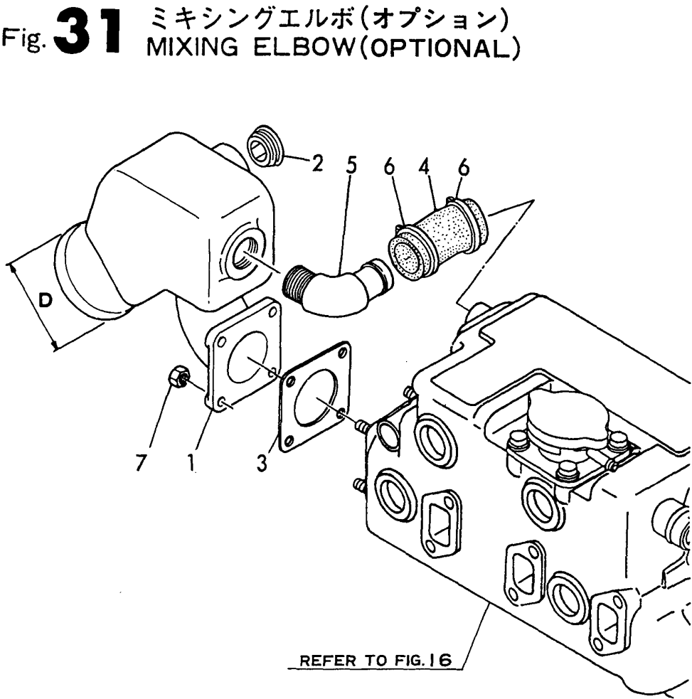
Fig.31.MIXING ELBOW(OPTIONAL)
