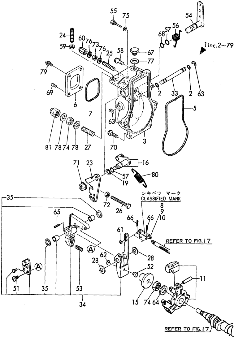
Fig. 22 ガバナ GOVERNOR
