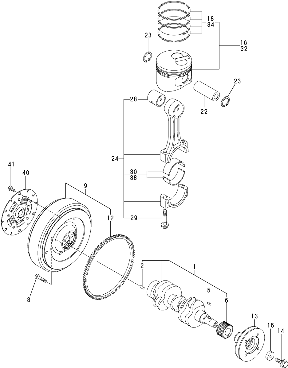
Fig.10.CRANKSHAFT & PISTON
