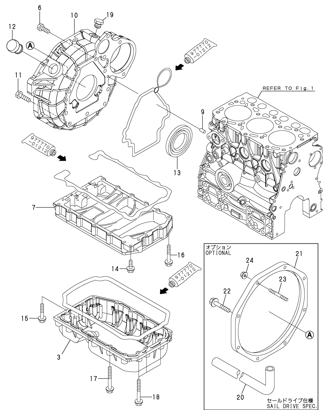
Fig.3.FLYWHEEL HOUSING & L.O.SUMP
