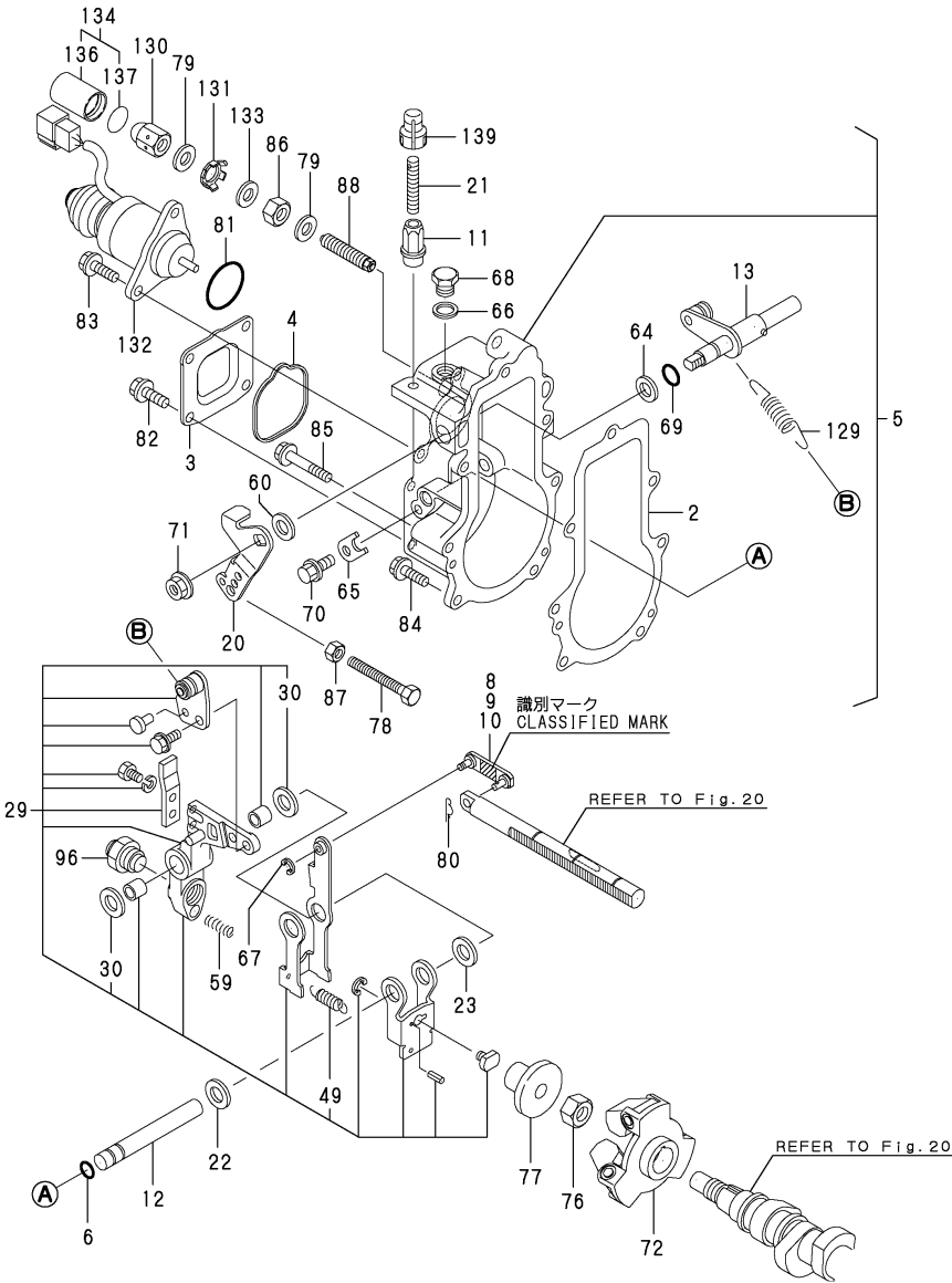
Fig.21.GOVERNOR
