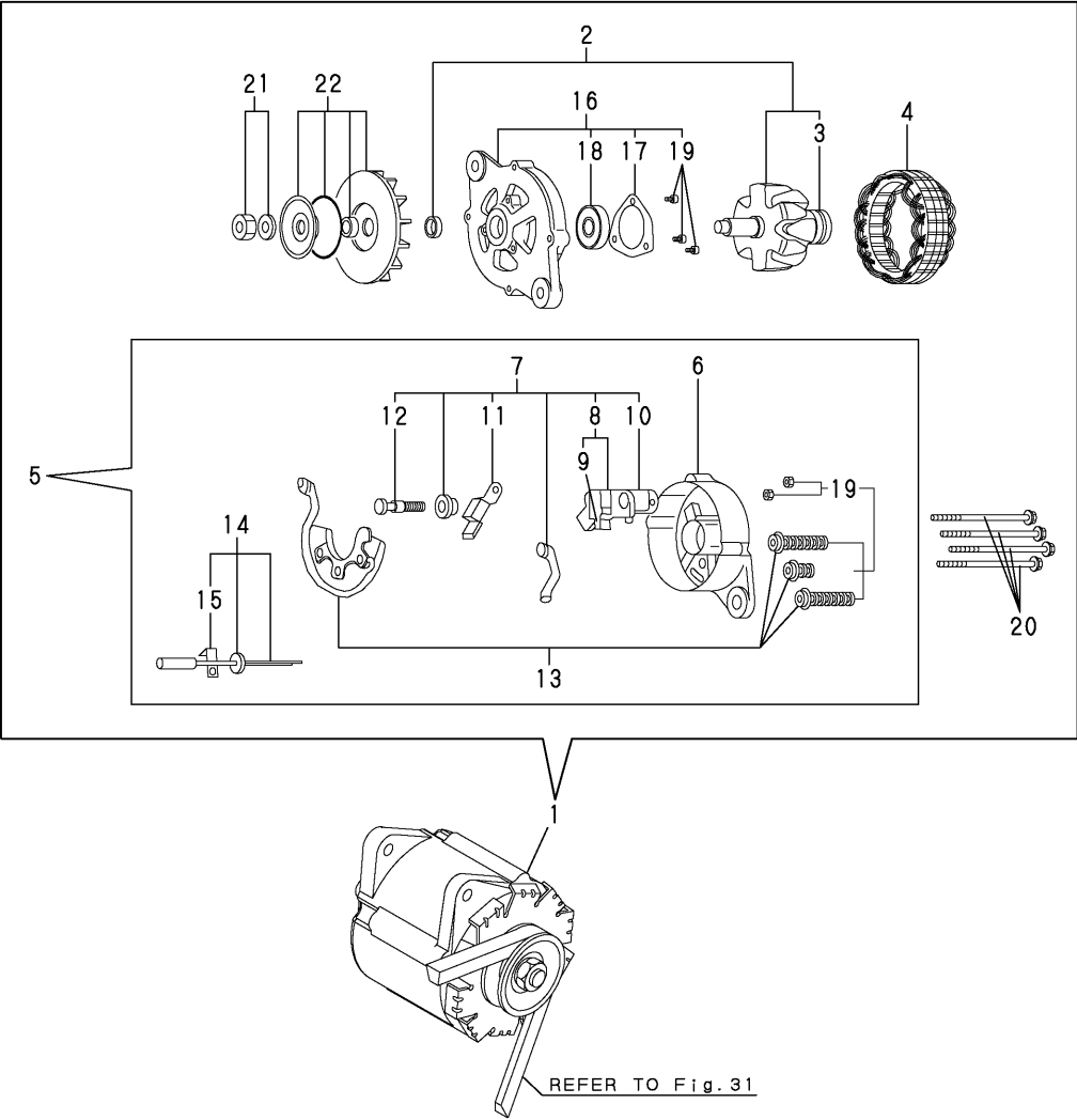
Fig.32.GENERATOR(80A/OPTIONAL)
