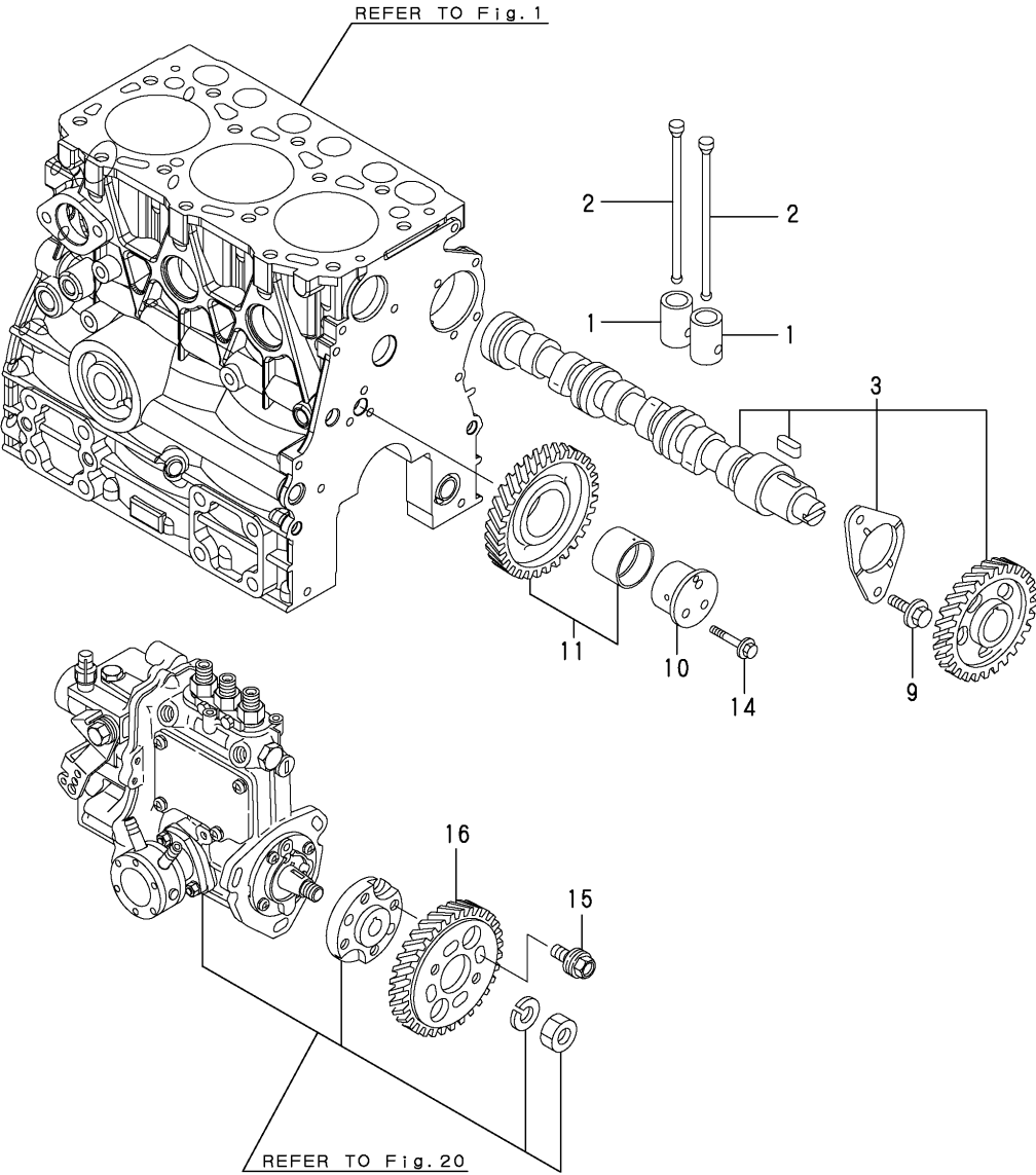
Fig.9.CAMSHAFT & DRIVING GEAR
