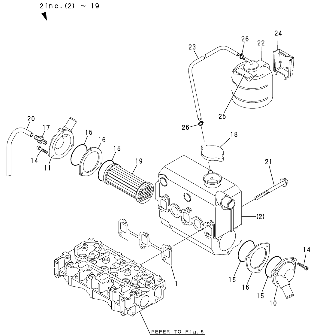
Fig.15.COOLING FRESH WATER COOLER
