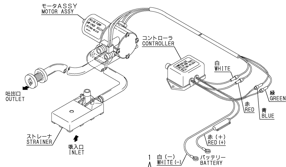
Fig.18.BILGE PUMP(STD/OPTIONAL)
