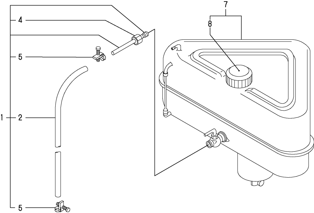
Fig.25.FUEL TANK(OPTIONAL)
