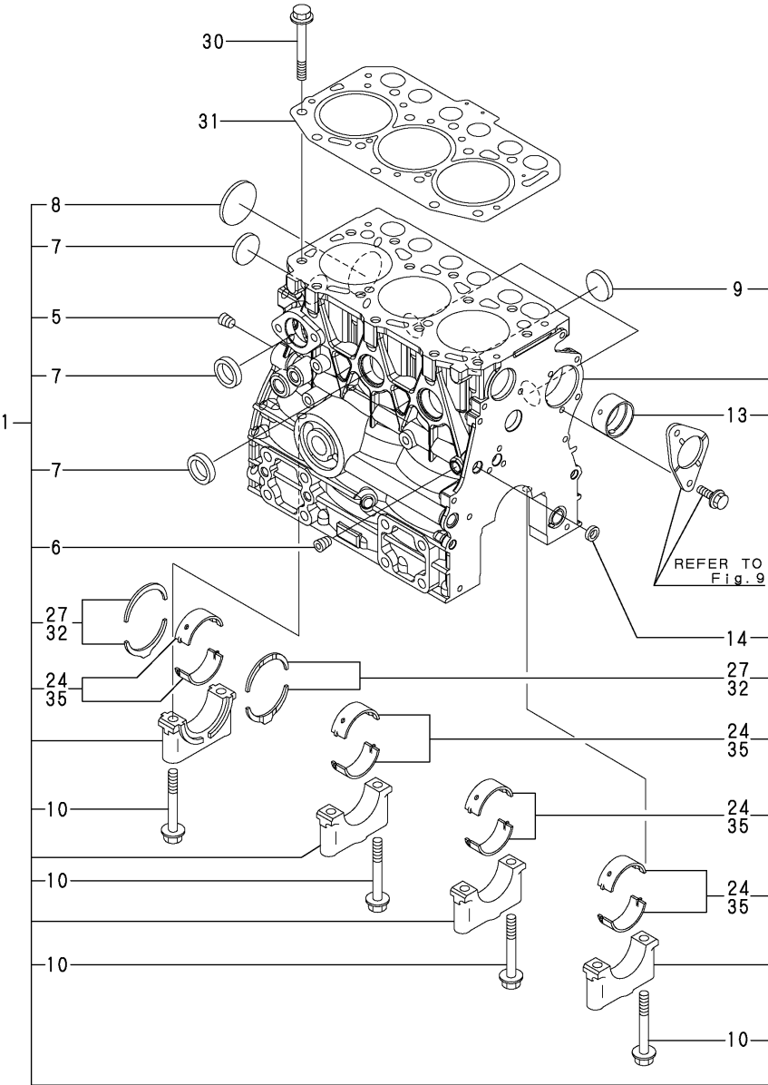
Fig.1.CYLINDER BLOCK
