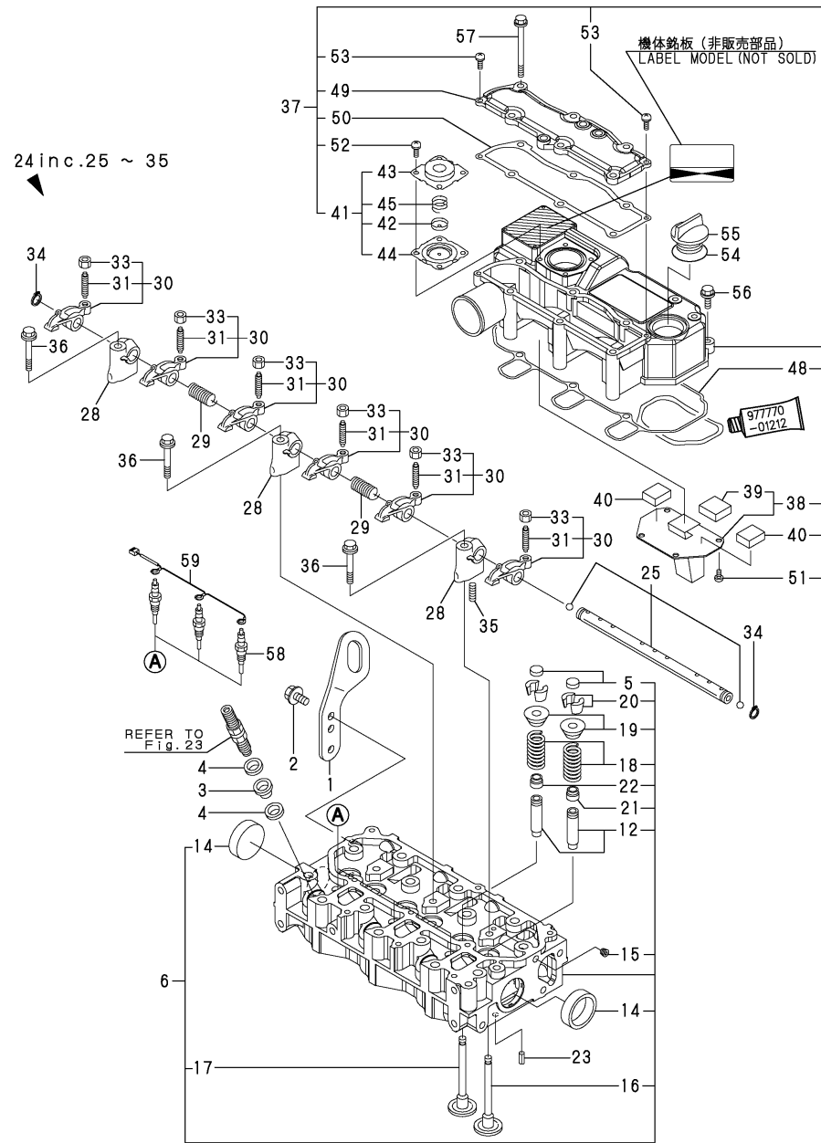
Fig.6.CYLINDER HEAD & BONNET
