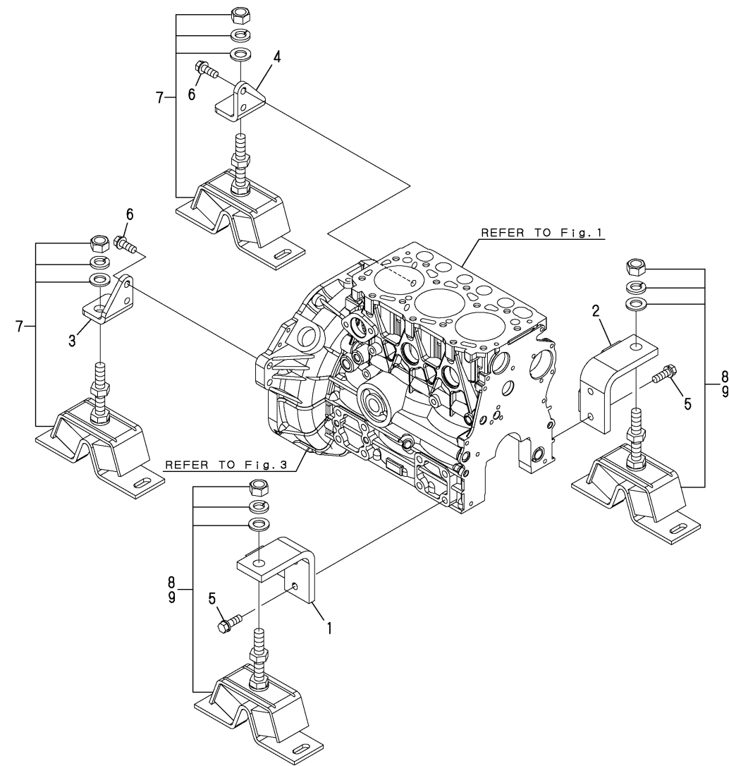
Fig.4.MOUNTING FOOT
