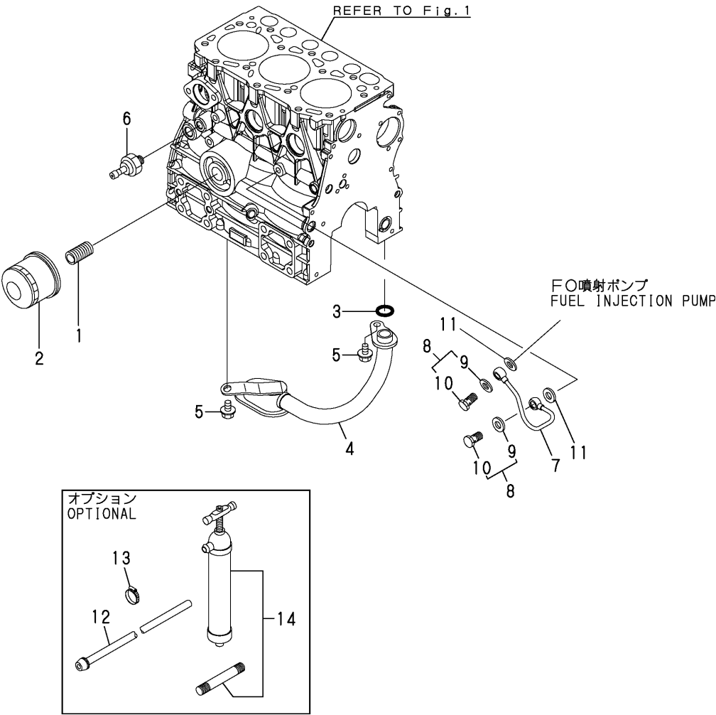
Fig.12.LUB.OIL SYSTEM
