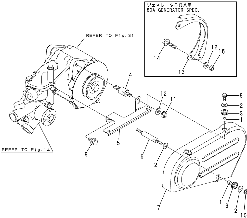
Fig.33.V-BELT COVER
