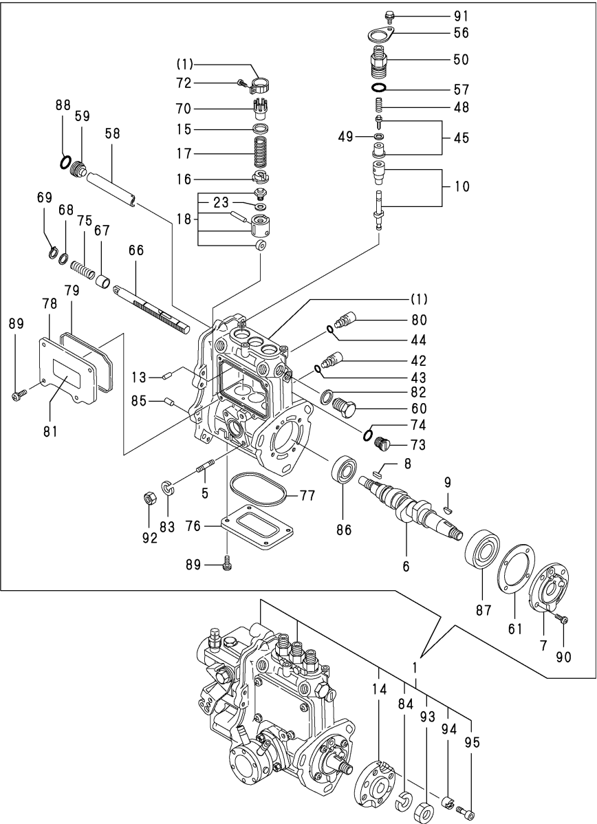
Fig.20.FUEL INJECTION PUMP
