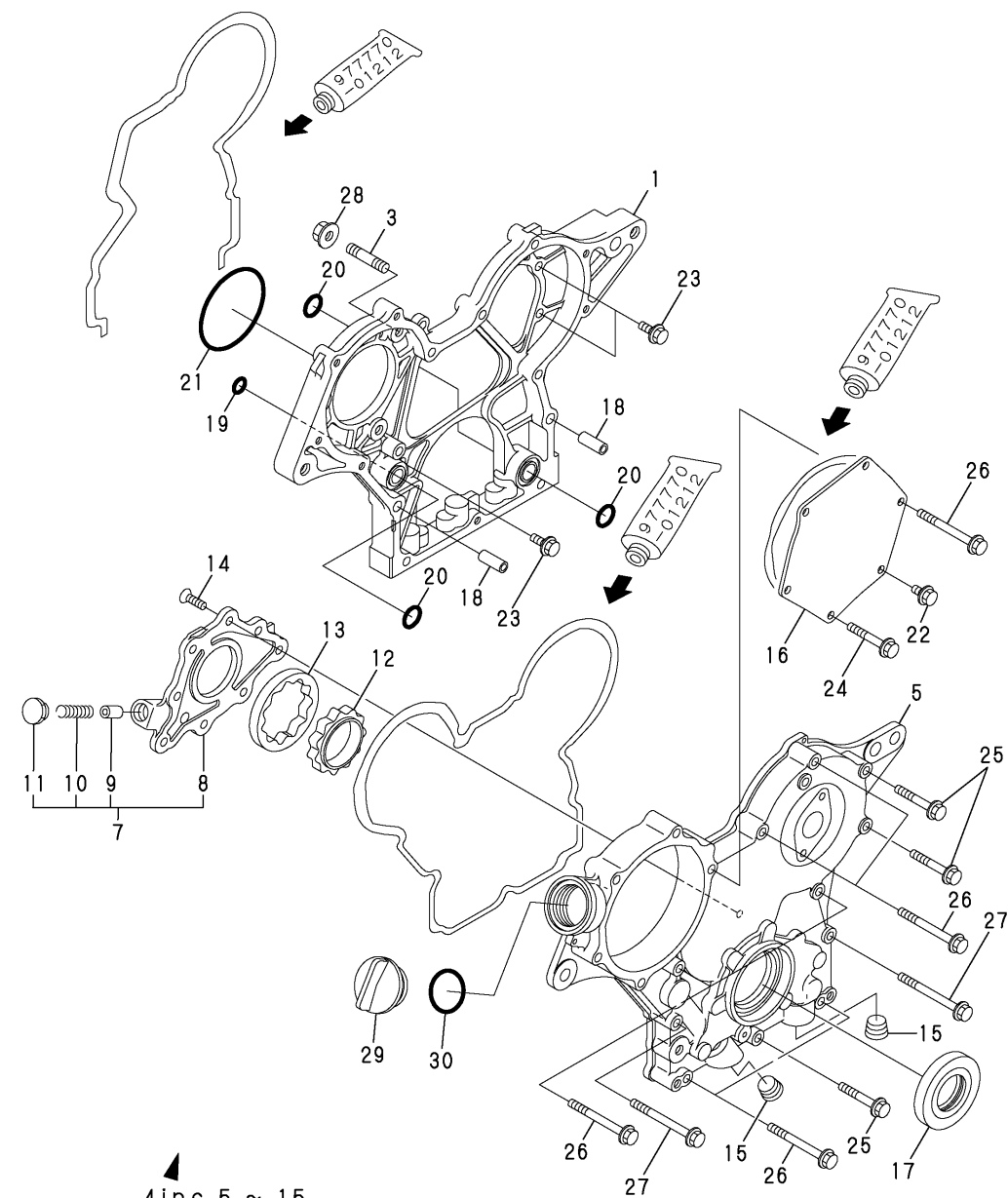
Fig.2.GEAR HOUSING
