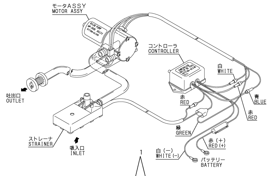
Fig.19.BILGE PUMP(DX/OPTIONAL)
