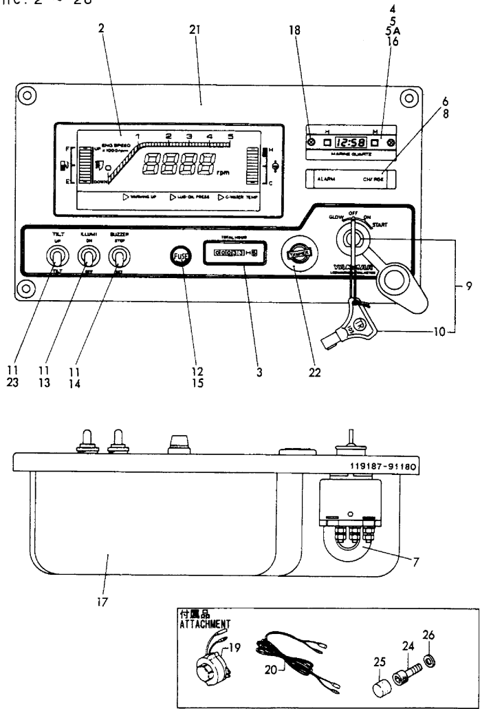
計器盤 (旧形, 4LH-HTZAY) INSTRUMENT PANEL (PREVIOUS, 4LH-HTZAY)
