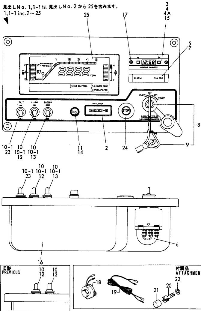
Fig.88 計器盤 (旧形, 4LH-HTZ/DTZ) INSTRUMENT PANEL (PRVIOUS, 4LH-HTZ/DTZ)
