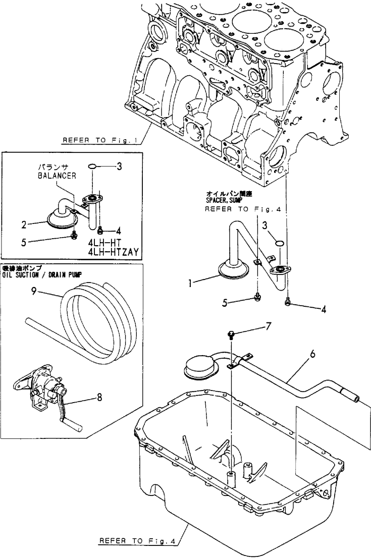
Fig.30 潤滑油吸入パイプ LUB.OIL SUCTION PIPE
