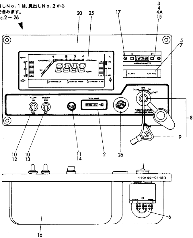
Fig.87 計器盤 (旧形, 4LH-HT) INSTRUMENT PANEL (PRVIOUS, 4LH-HT)
