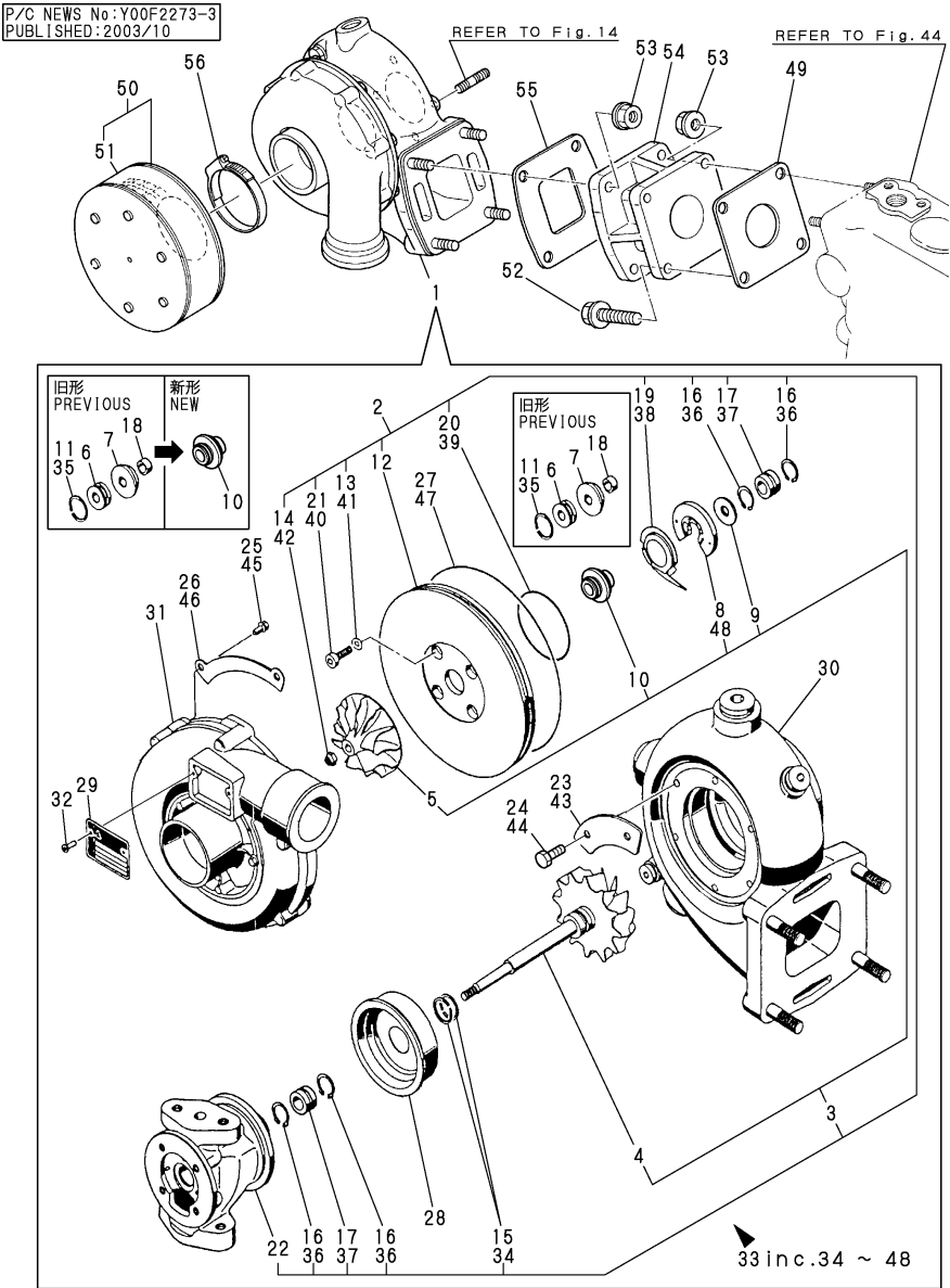
Fig.18.TURBOCHARGER(4LH-DTZ)
