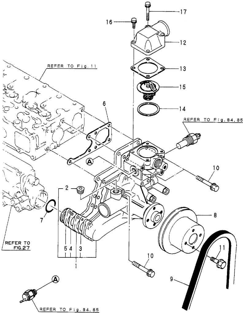
Fig.42 冷却水ポンプ (清水) COOLING FRESH WATER PUMP
