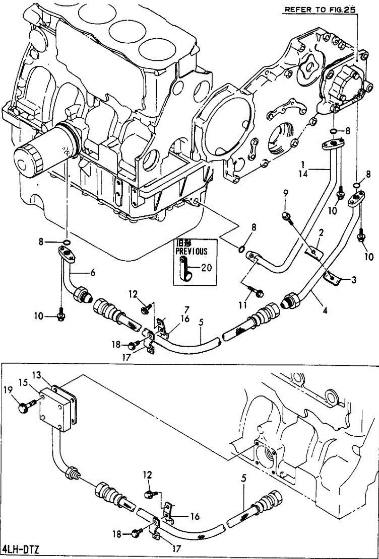
Fig.35 潤滑油パイプ (サブ) LUB.OIL PIPE (SUB)
