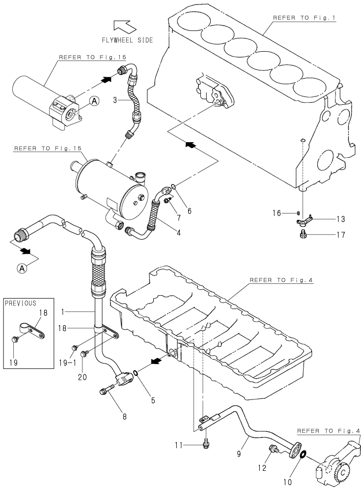
Fig.16 LUB.OIL PIPE & NOZZLE
