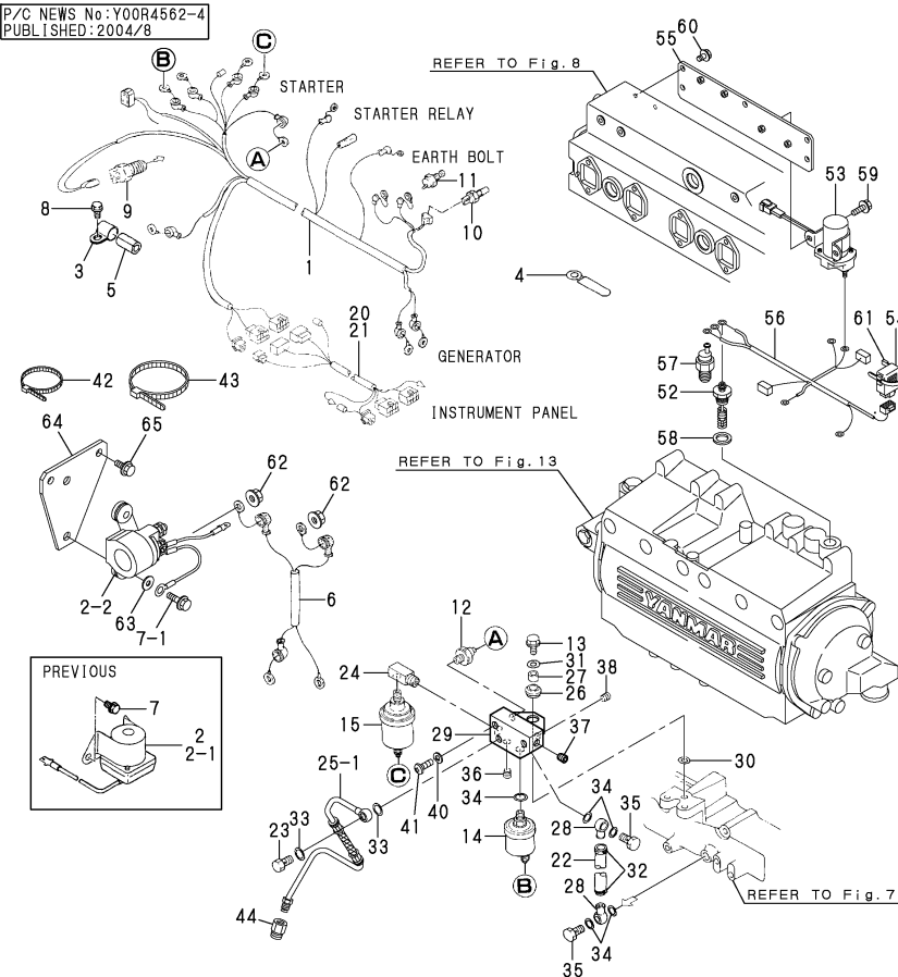
Fig.36.WIRE HARNESS & SENSOR
