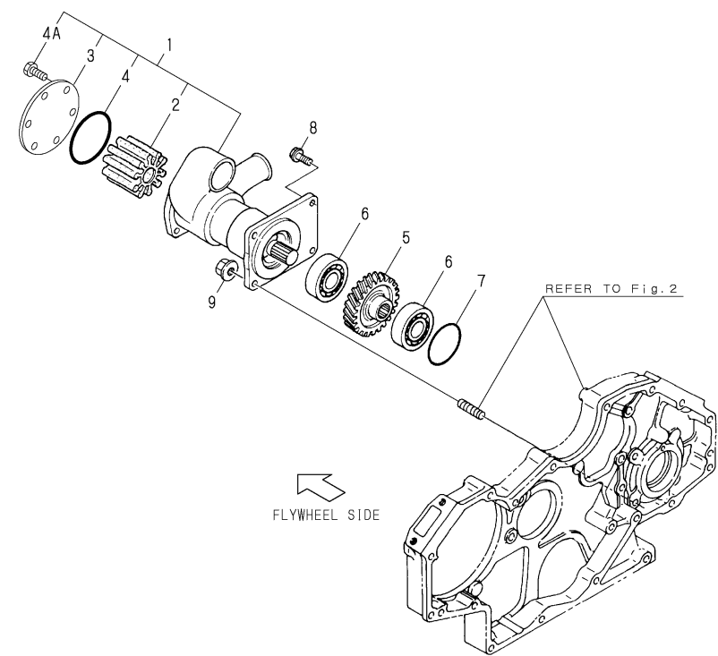
Fig.21 COOLING SEA WATER PUMP
