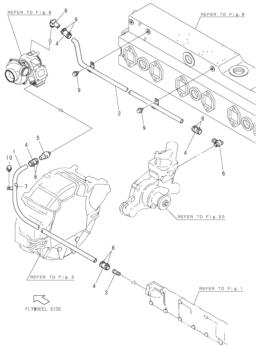
Fig.24 C.F.W. PIPE (TURBOCHARGER)
