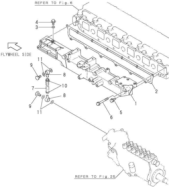
Fig.7 SUCTION MANIFOLD
