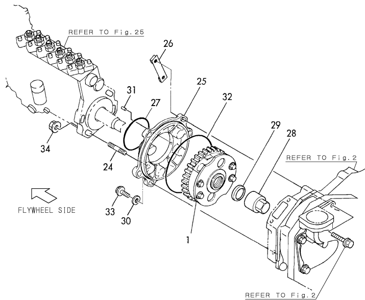
Fig.28 TIMER
