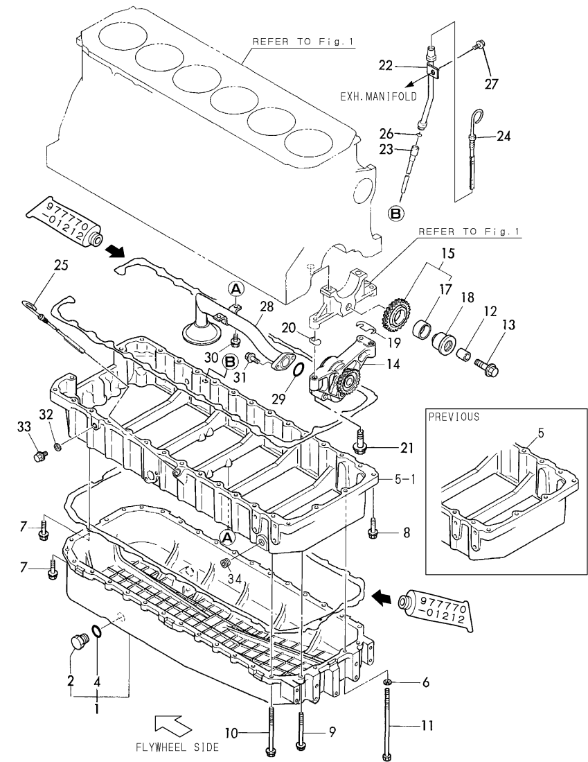
Fig.4 LUB.OIL SUMP & LUB.OIL PUMP
