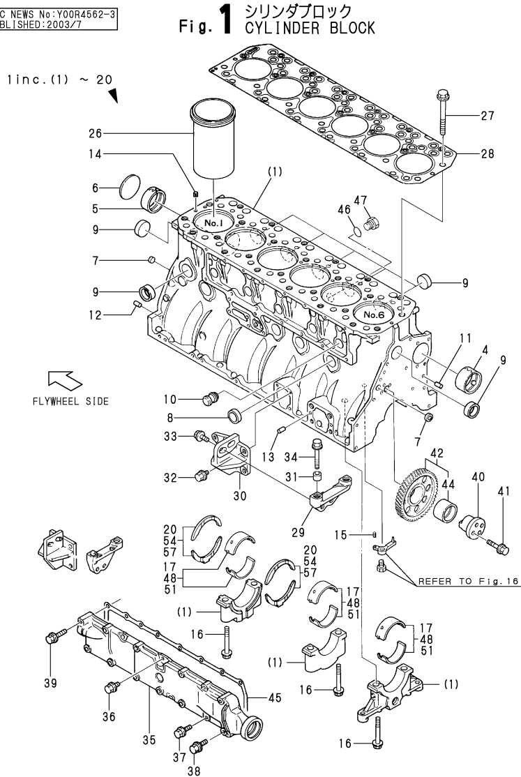
Fig.1.CYLINDER BLOCK
