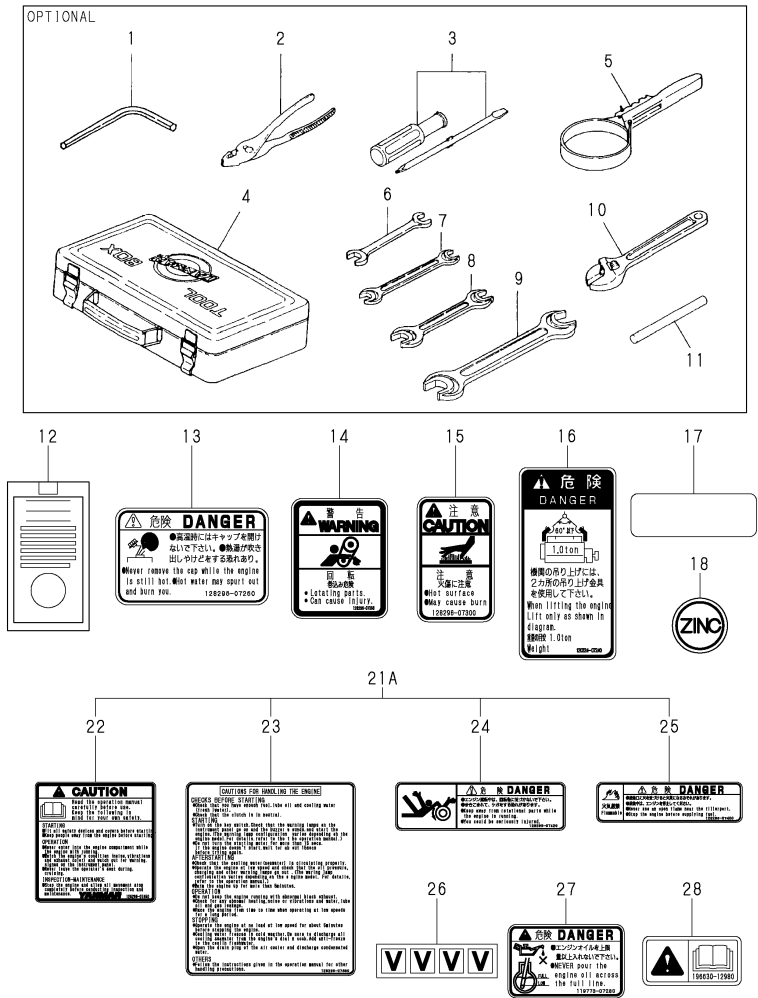
Fig.52 TOOL & LABEL
