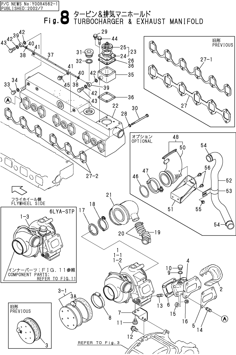
Fig.8.TURBOCHARGER & EXHAUST MANIFOLD
