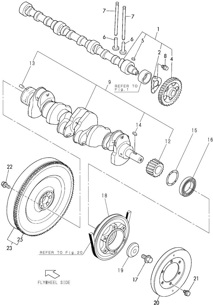
Fig.12 CAMSHAFT & CRANKSHAFT
