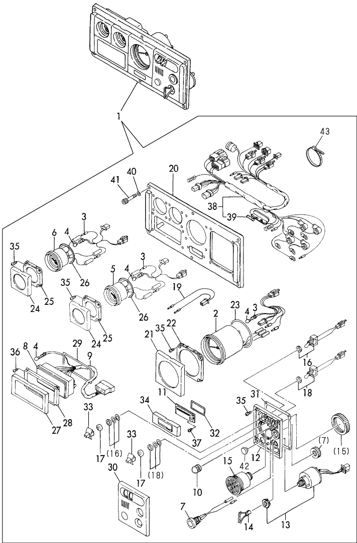
Fig. 47 INSTRUMENT PANEL (C-TYPE, OPTIONAL, NEW)
