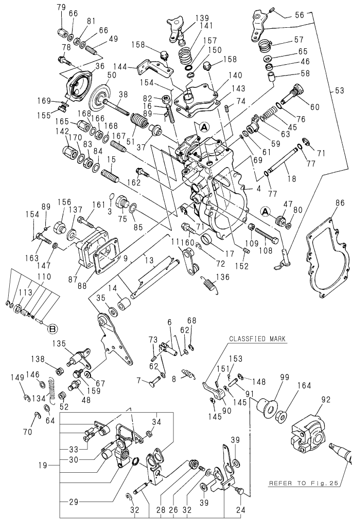
Fig. 26 GOVERNOR
