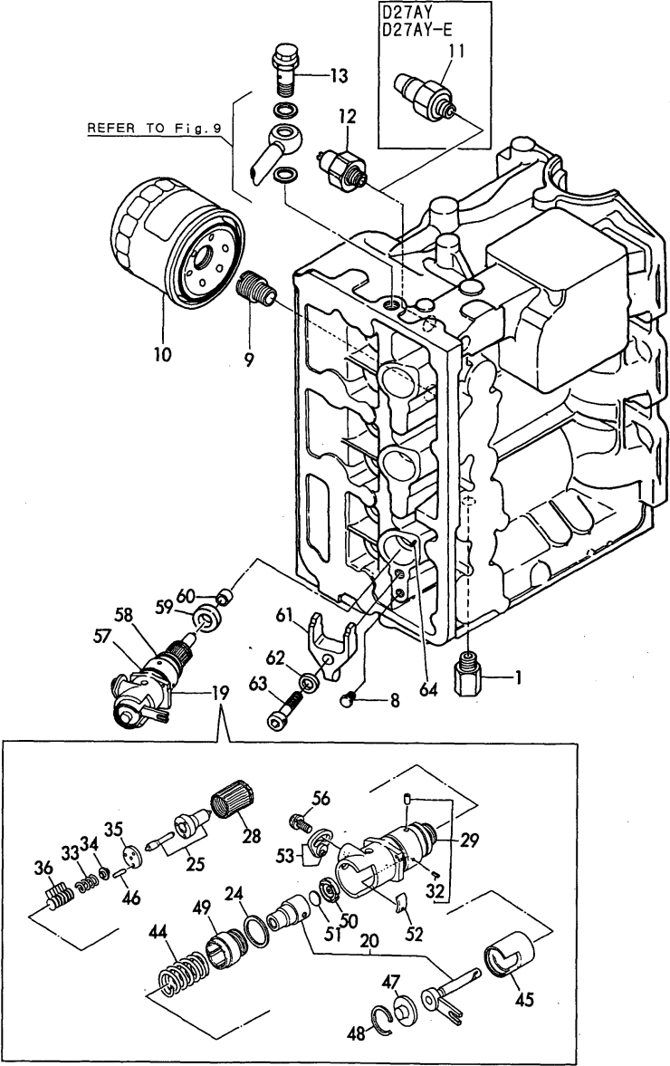
Fig.8 潤滑油フィルタ&調圧弁 LUB.OIL STRAINER & PRESS.CONTROL VALVE
