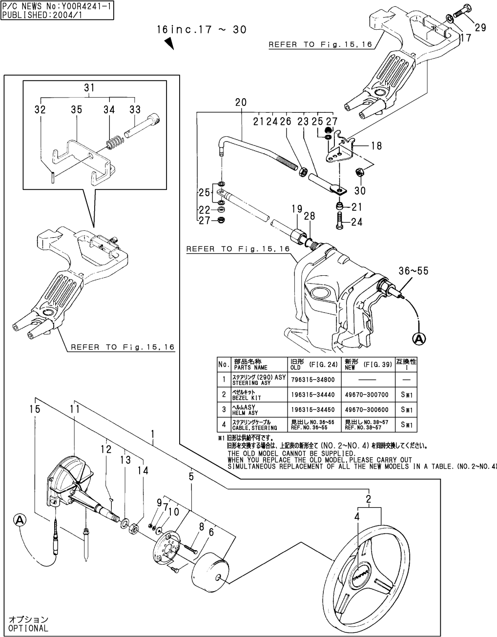
Fig.24.STEERING REMO-CON(PREVIOUS)
