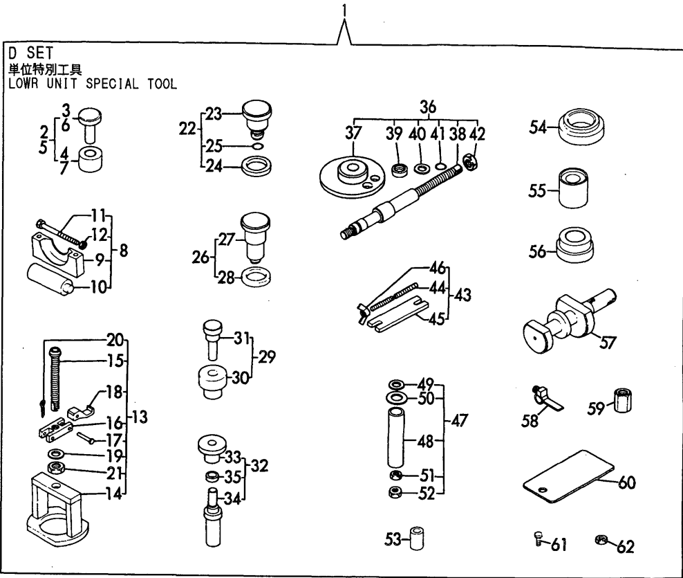
Fig.28 特殊工具 (2) (オプション) SPECIAL TOOL (2) (OPTIONAL)
