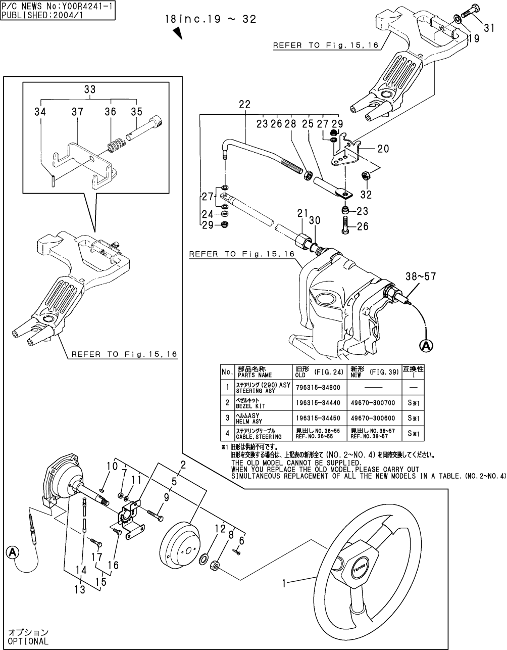
Fig.39.(24A)STEERING REMO-CON(NEW)
