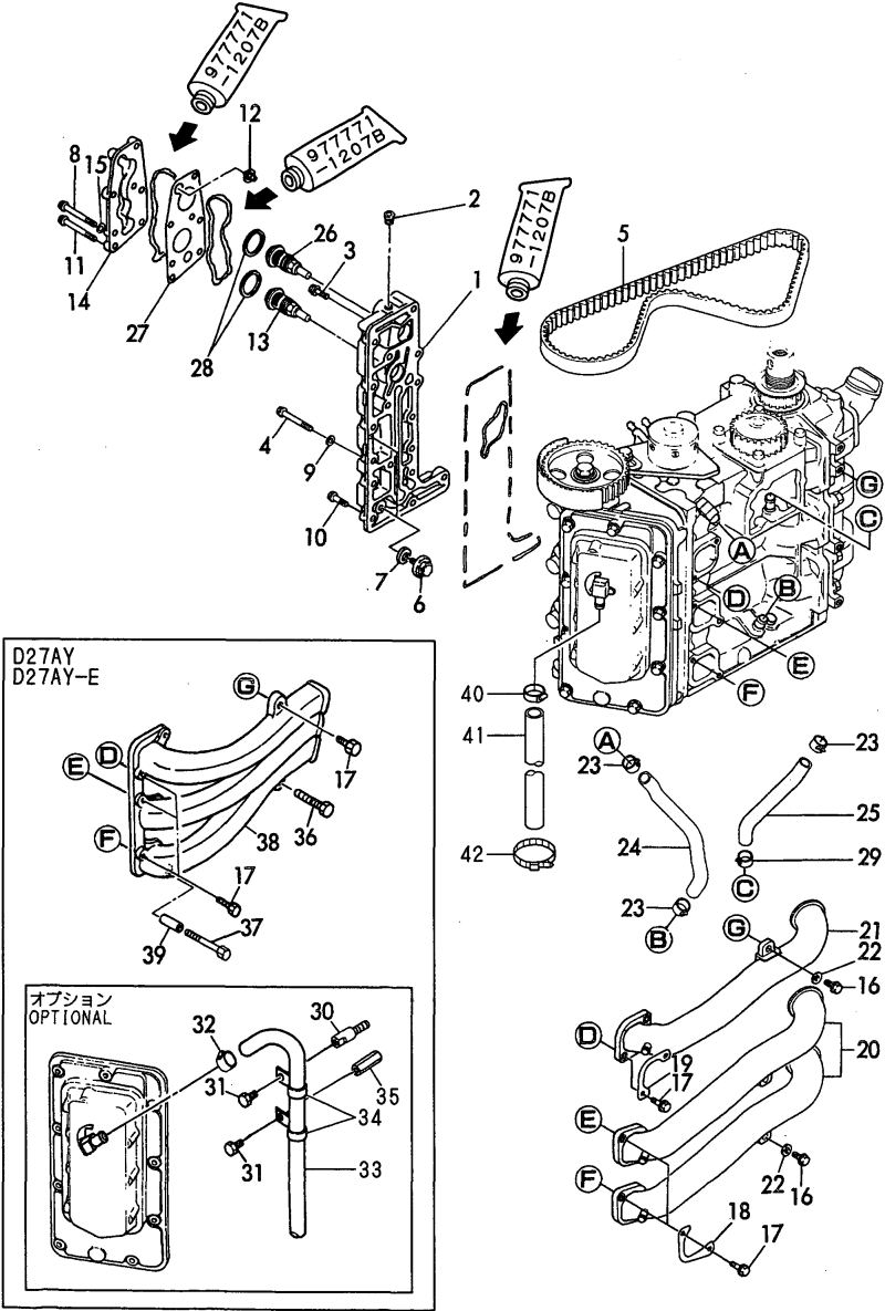
Fig.2 側蓋&吸気パイプ SIDE COVER & INTAKE PIPE
