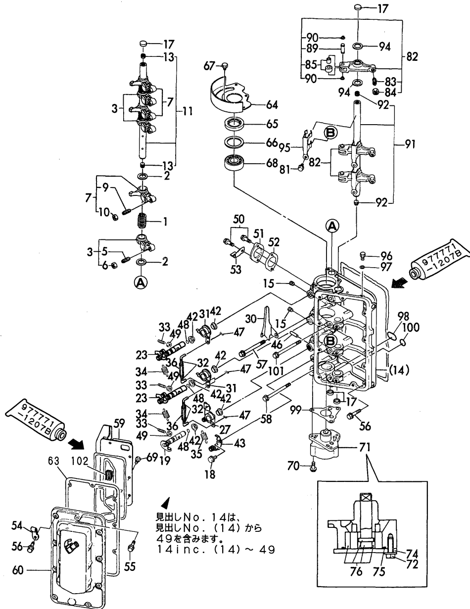
Fig. 4 BONNET & LUB.OIL PUMP
