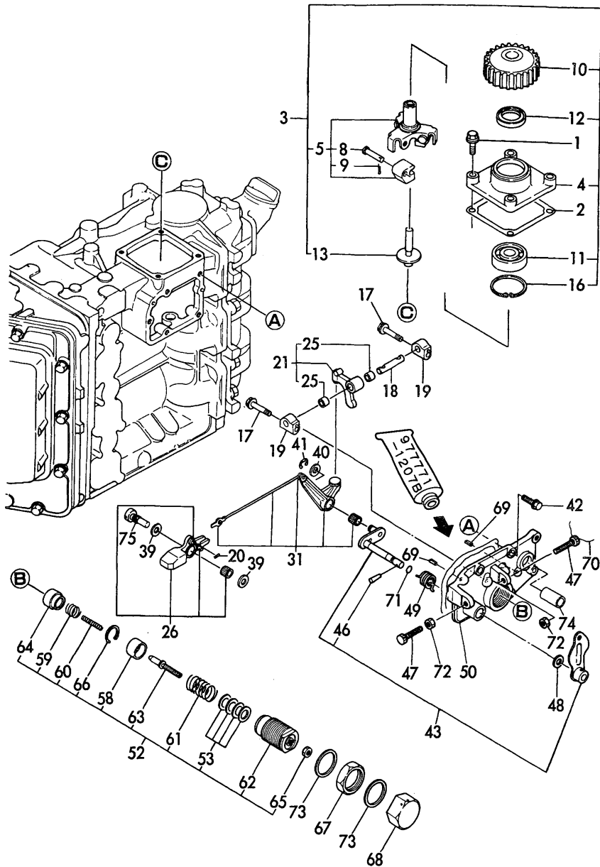
Fig.10 ガバナ&ガバナレバー GOVERNOR & GOVERNOR LEVER
