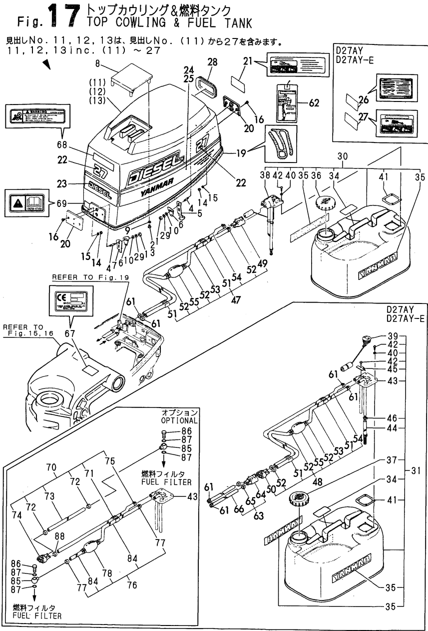
Fig.17.TOP COWLING & FUEL TANK
