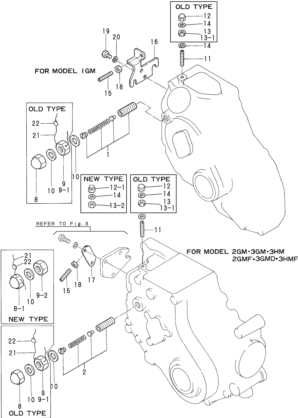
Fig.41.FUEL CONTROLLER
