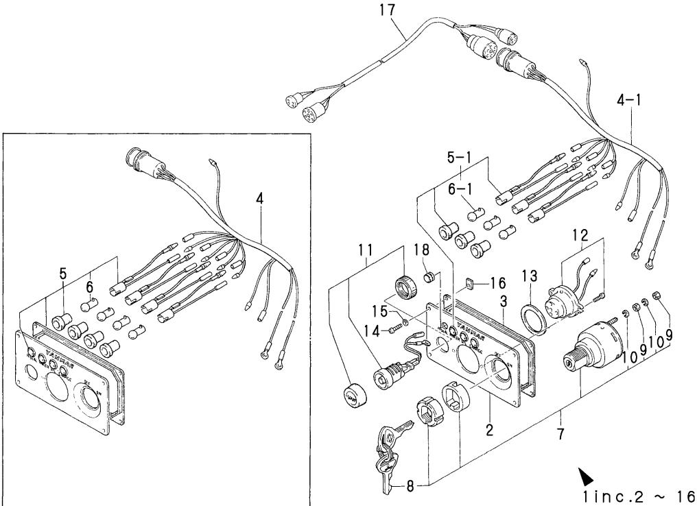
Fig.62.INSTRUMENT PANEL(S-TYPE/OPTIONAL)
