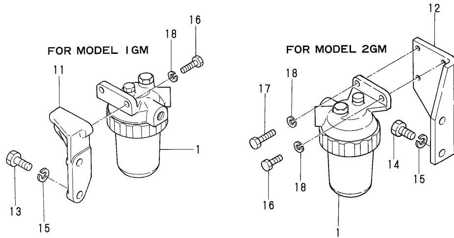
Fig.37.FUEL STRAINER
