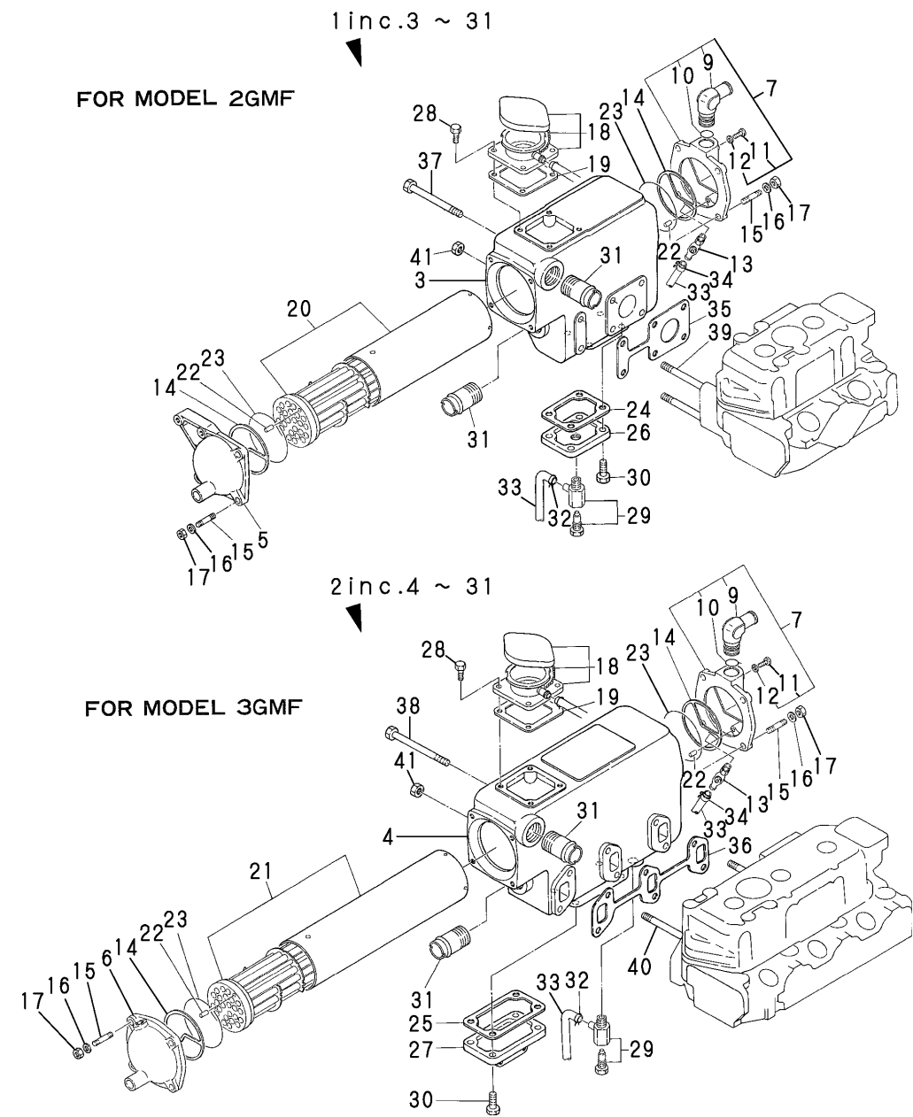
Fig.28.COOLING FRESH WATER COOLER
