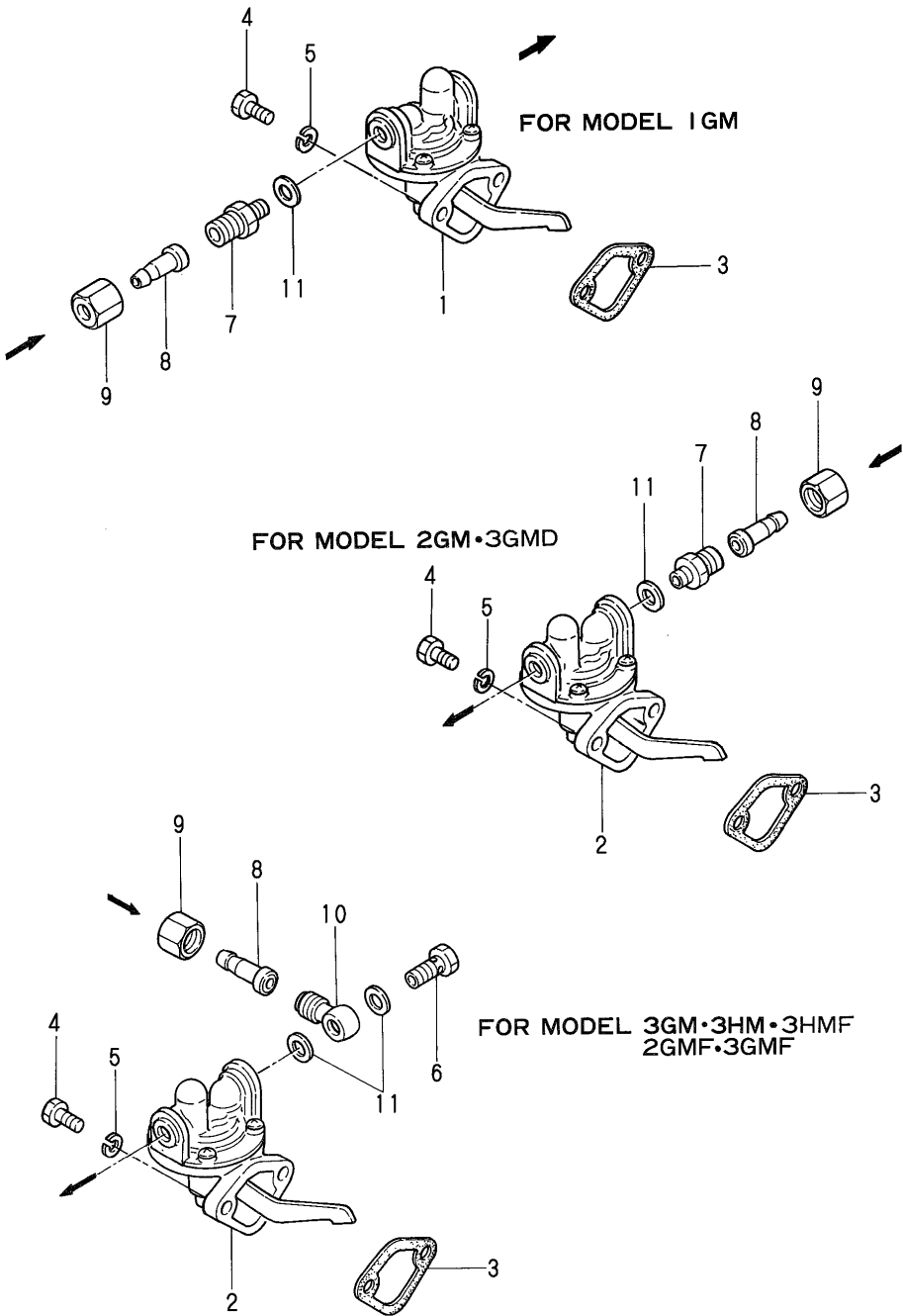
Fig.35.FUEL FEED PUMP
