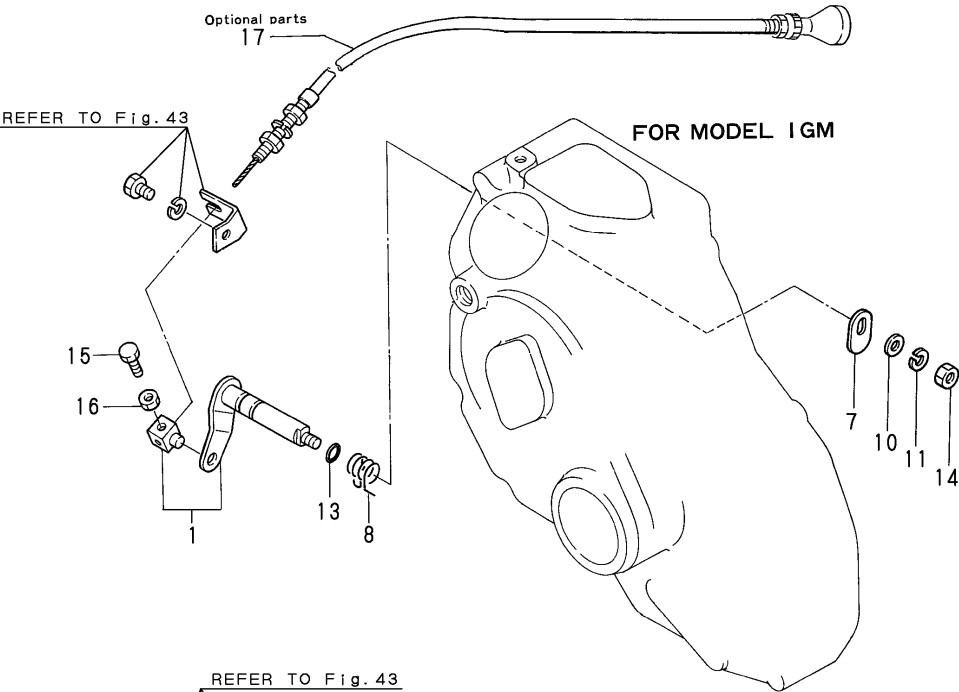
Fig.42.ENGINE STOP DEVIC
