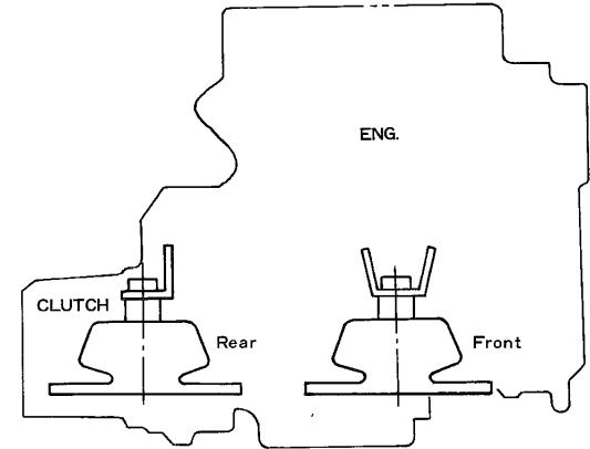
Fig.56.FLEXIBLE MOUNTING(OPTIONAL)
