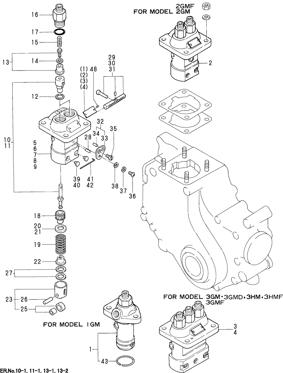
Fig.34.FUEL INJECTION PUMP
