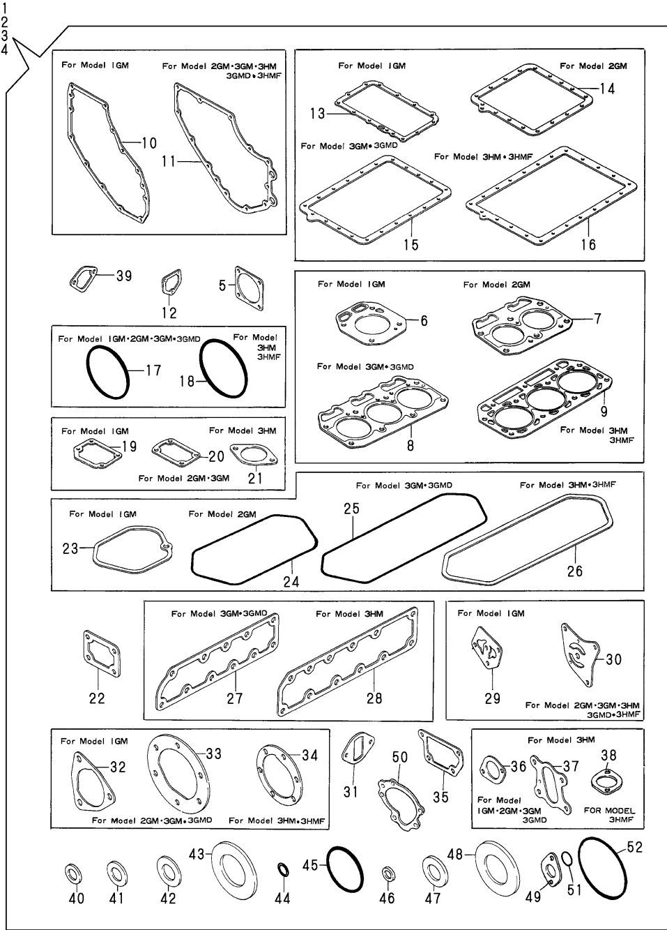
Fig.65.GASKET KIT(OPTIONAL)
