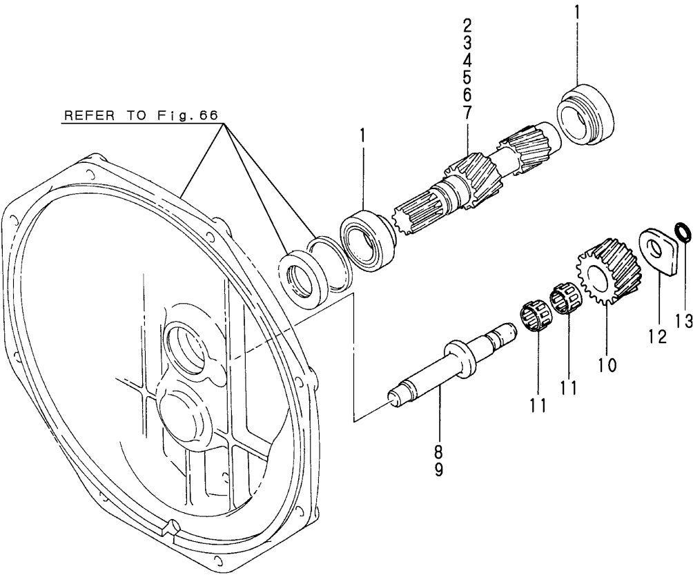
Fig.67.INPUT SHAFT & IDLE GEAR SHAFT
