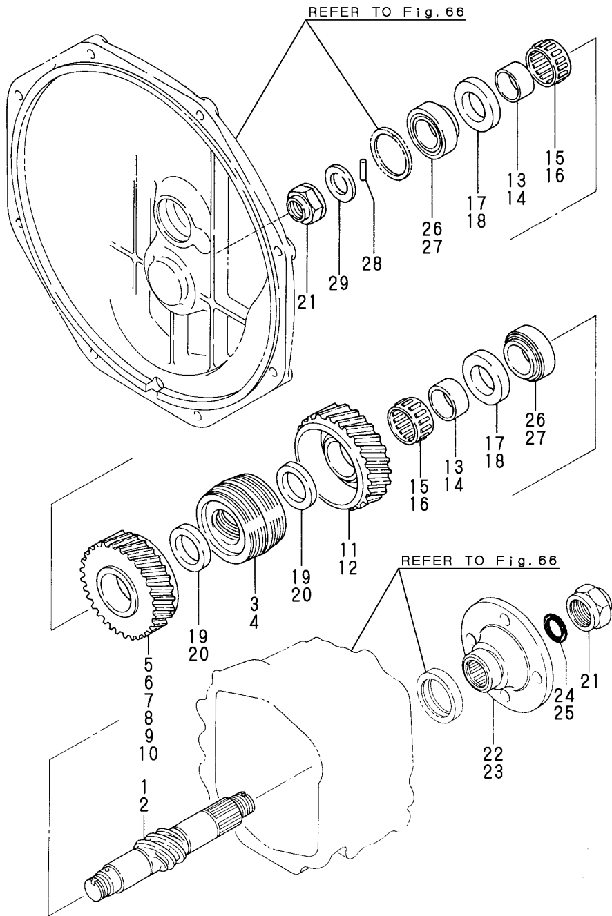
Fig.68.OUTPUT SHAFT
