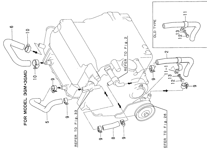
Fig.31.COOLING WATER PIPE
