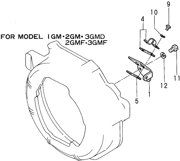
Fig.54.CLUTCH REMOTE CONTROL
