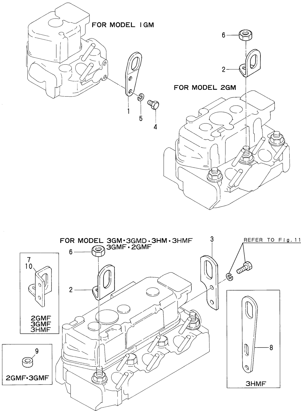
Fig.9.ENGINE LIFTER
