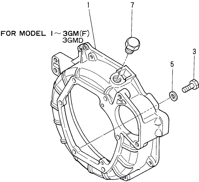
Fig.4.FLYWHEEL HOUSING
