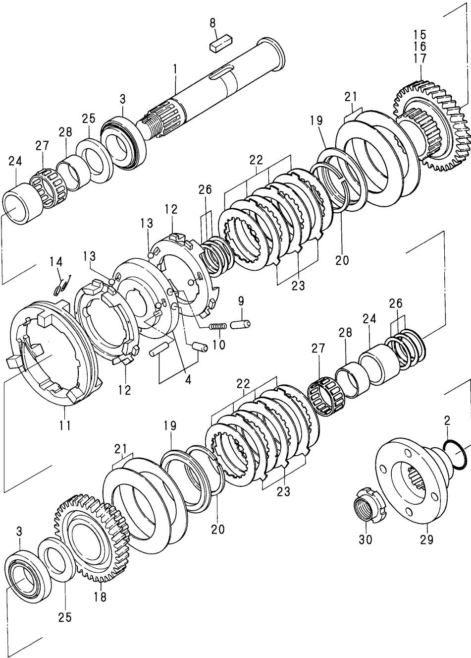
Fig.72.OUTPUT SHAFT
