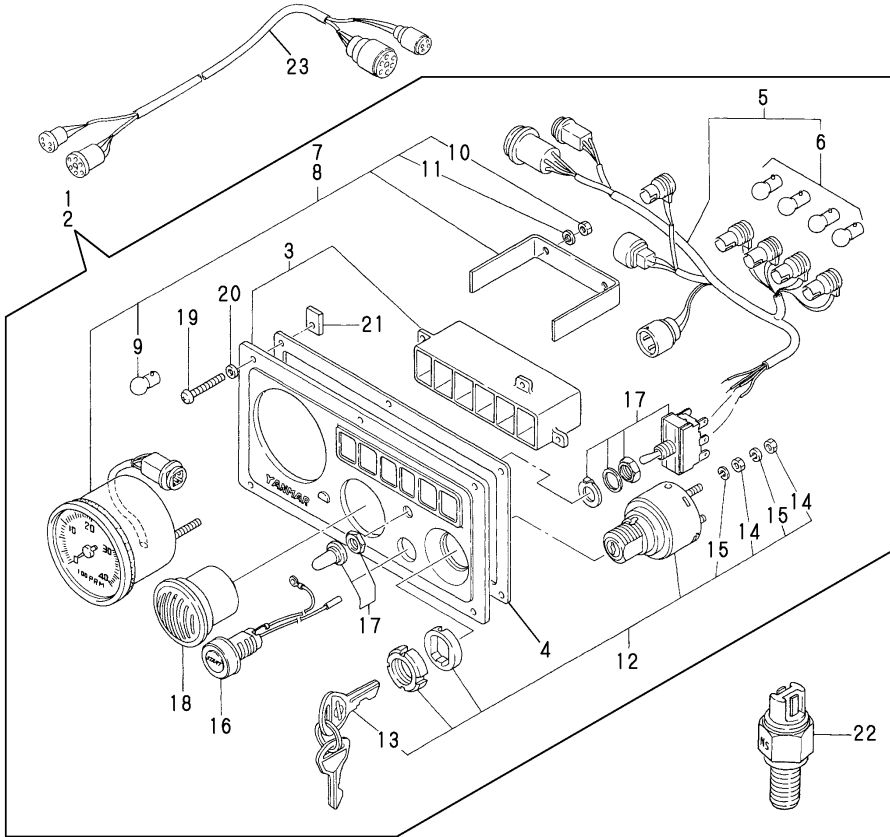
Fig.61.INSTRUMENT PANEL(M1 & M2-TYPE/-TYPE/OPTIONAL)
