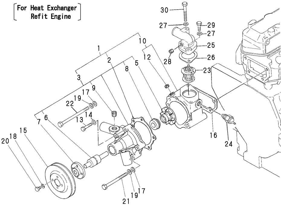
Fig.74.COOLING FRESH WATER PUMP & SUB-TANK
