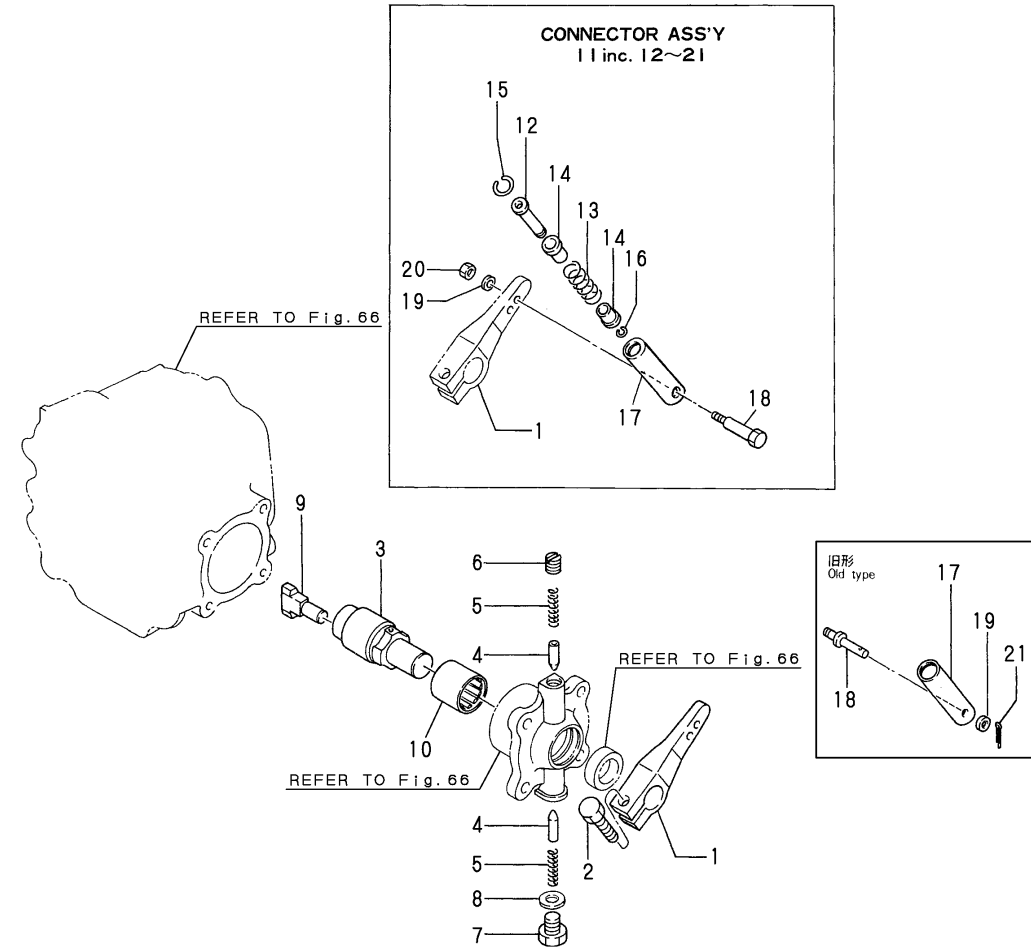
Fig.69.CONTROL DEVICE
