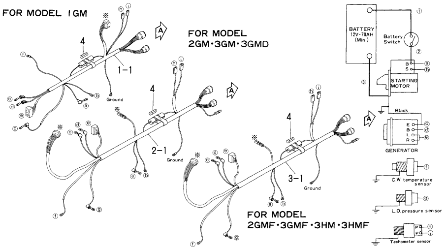
Fig.52.WIRE HARNESS
