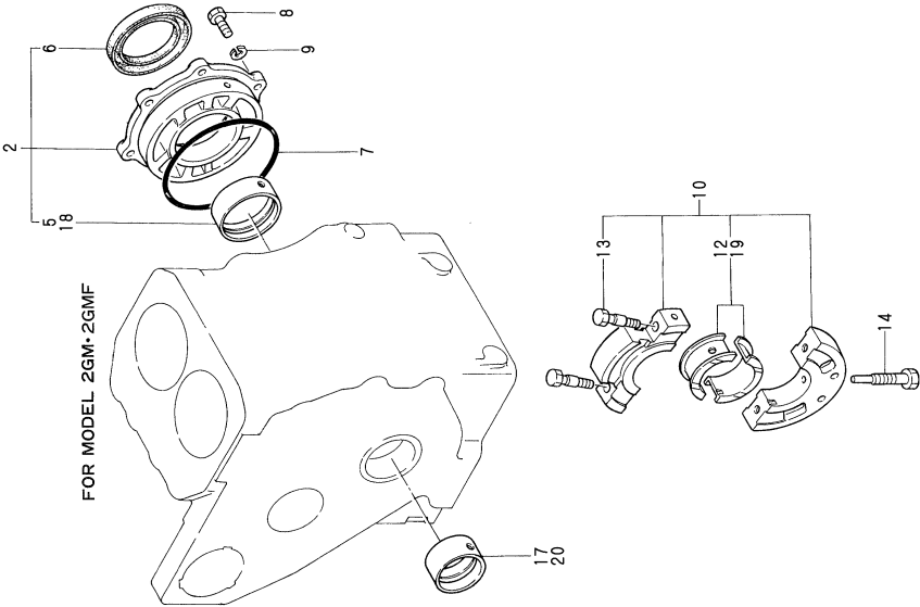
Fig.6.MAIN METAL HOUSING(1,2GM(F))
