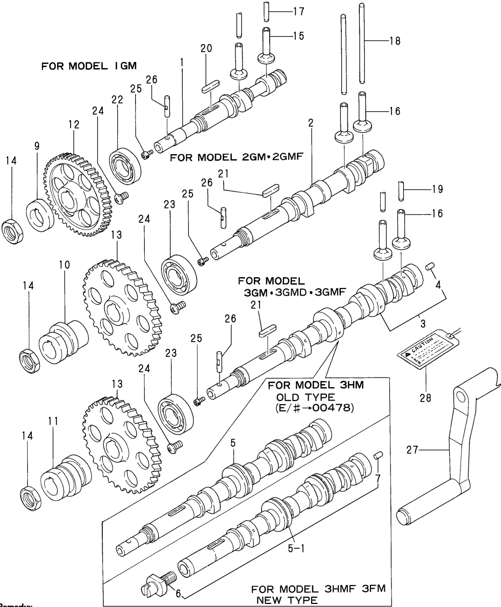
Fig.17.CAMSHAFT
