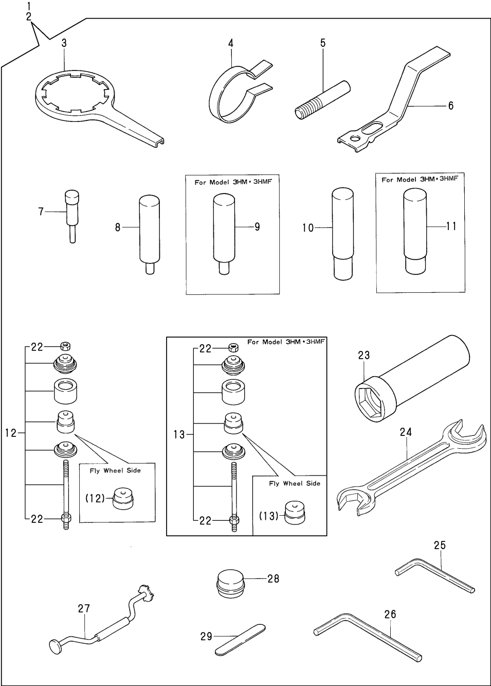
Fig.63.SPECIAL TOOL(OPTIONAL)
