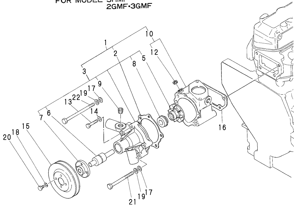
Fig.27.COOLING FRESH WATER PUMP
