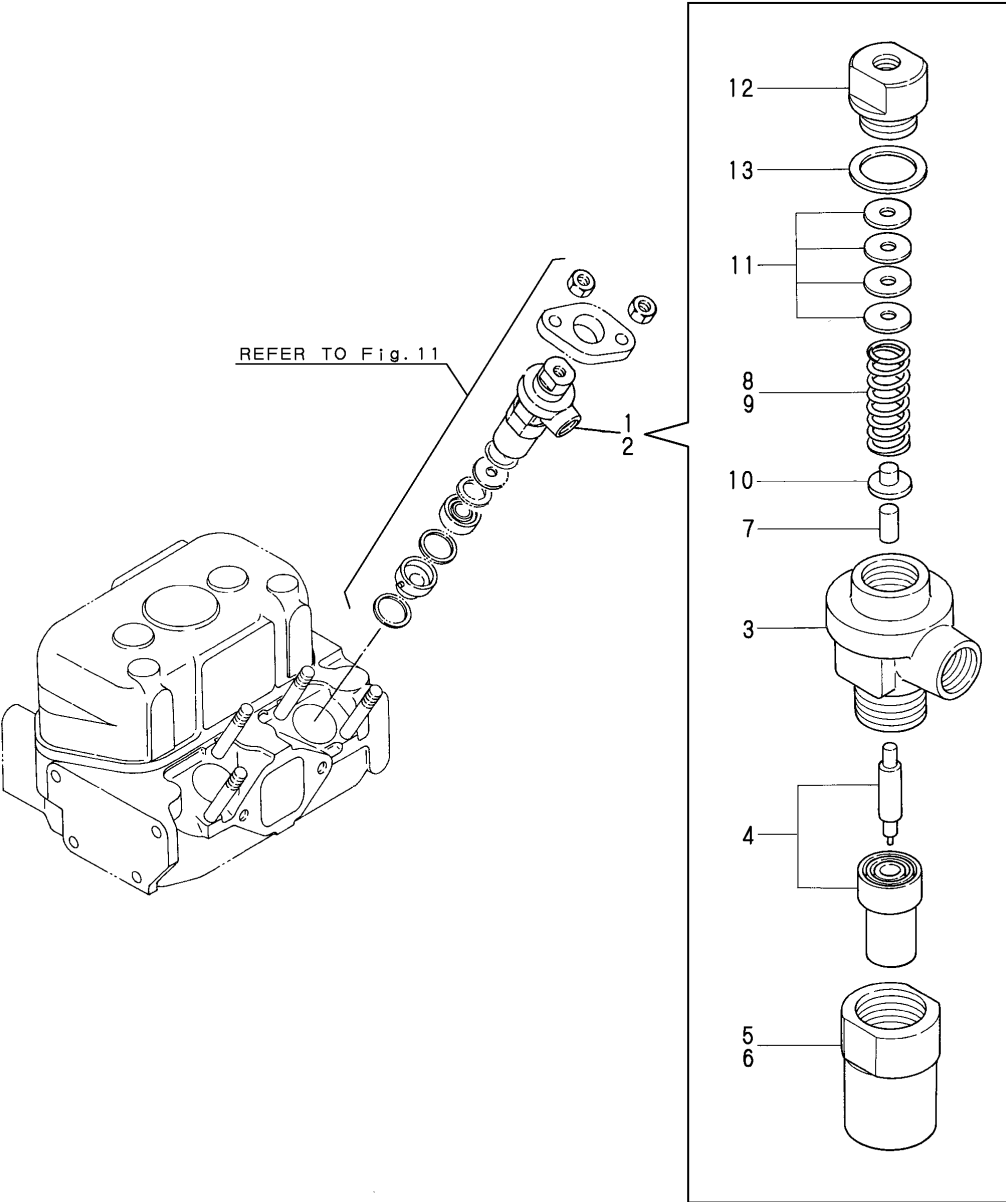
Fig.36.FUEL INJECTION VALVE
