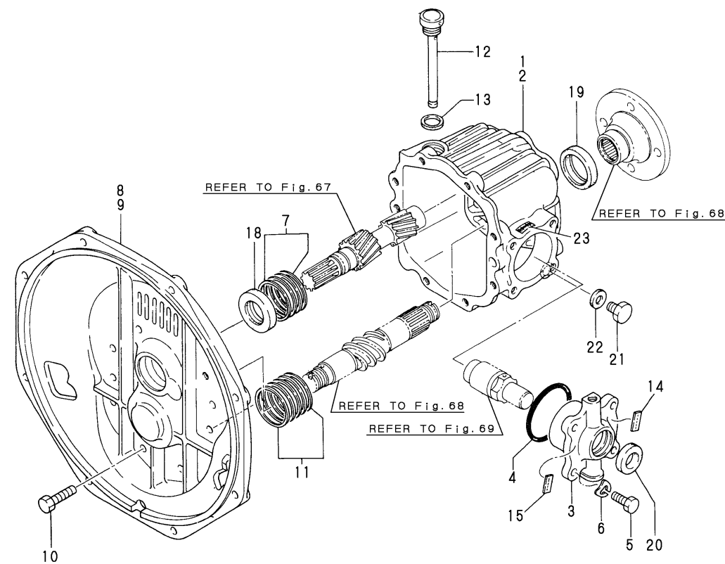
Fig.66.CLUTCH HOUSING
