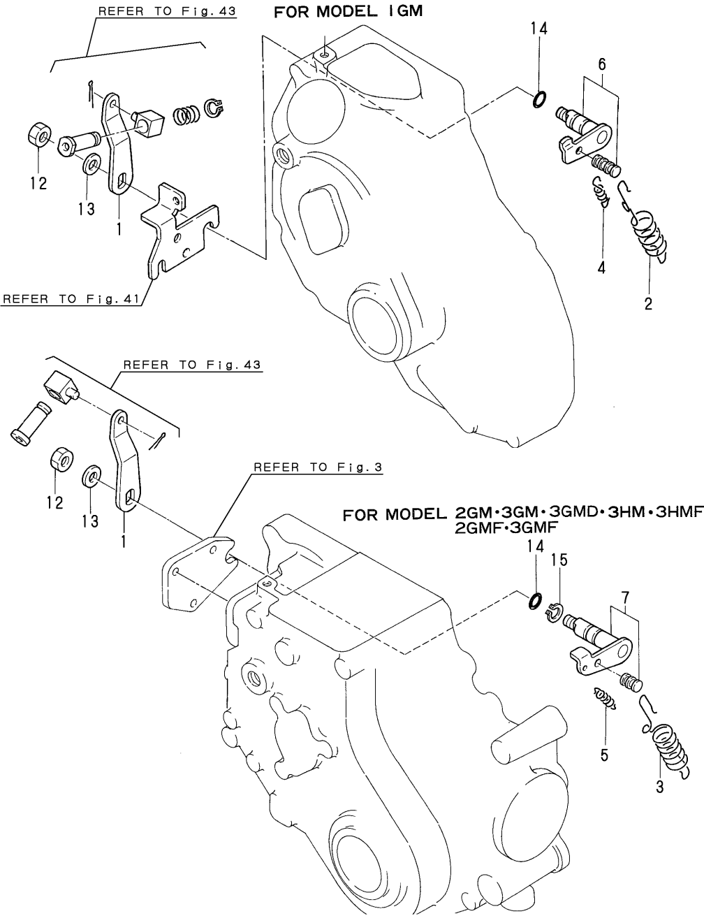
Fig.40.REGULATOR LINKS
