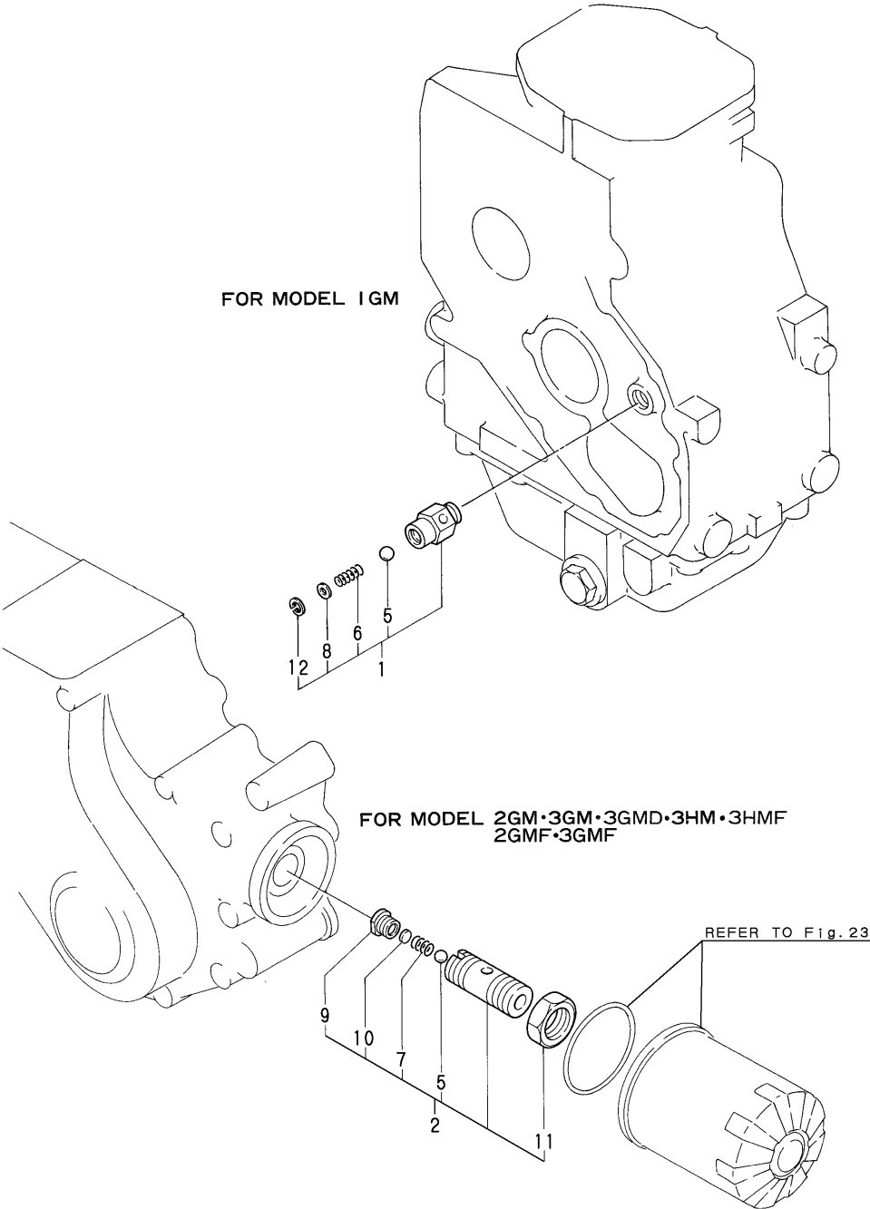
Fig.24.LUB.OIL PRESSURE CONTROL VALVE
