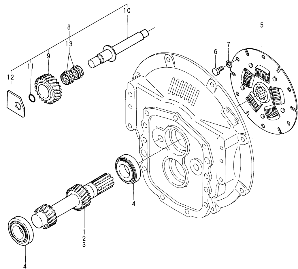
Fig.71.INPUT SHAFT & IDLE GEAR SHAFT
