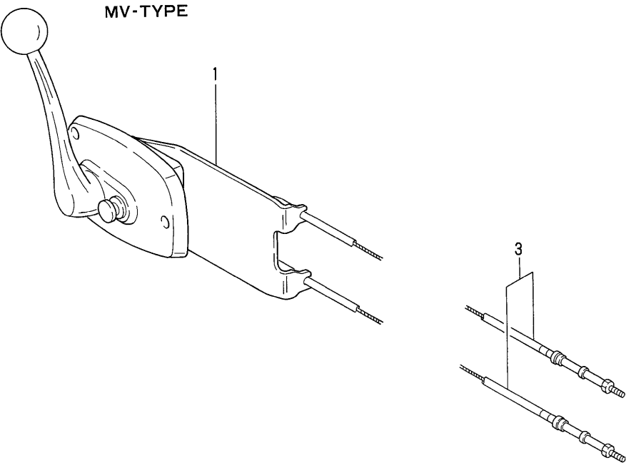
Fig.60.SINGLE LEVER CONTROL(OPTIONAL)
