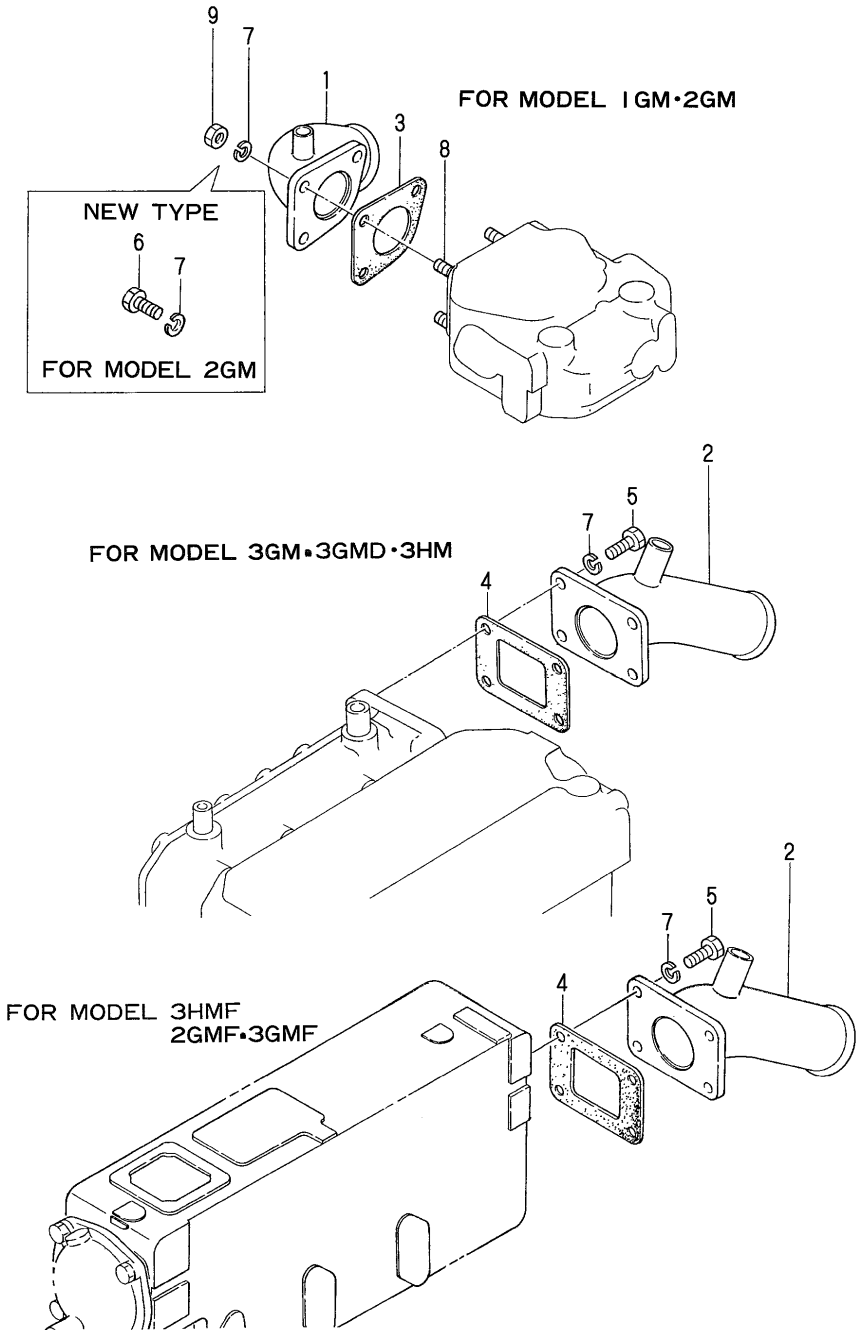
Fig.15.MIXING ELBOW
