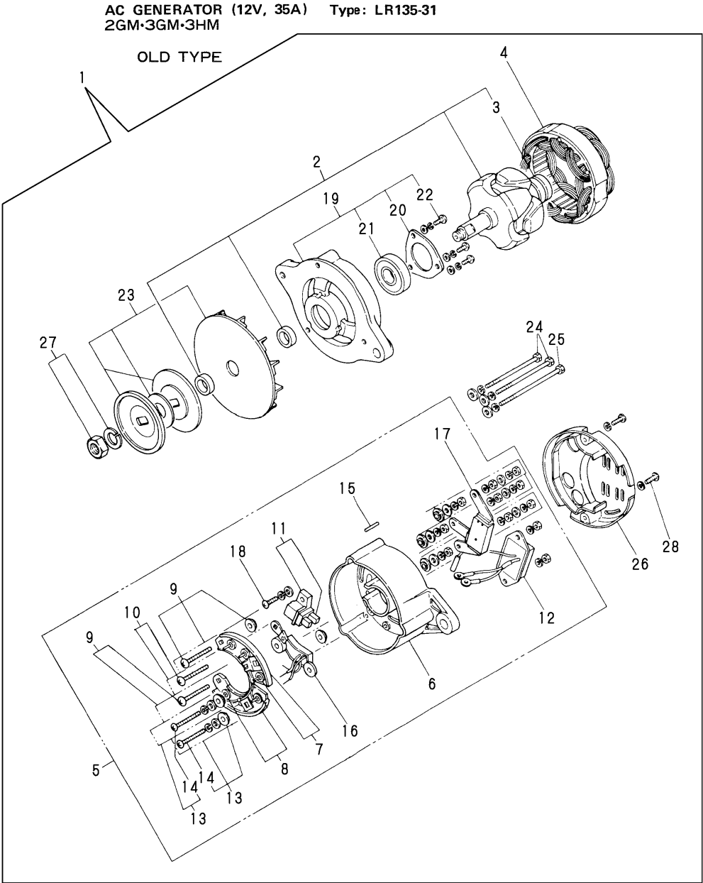
Fig.48.GENERATOR COMPONENT PART(121370-77200)
