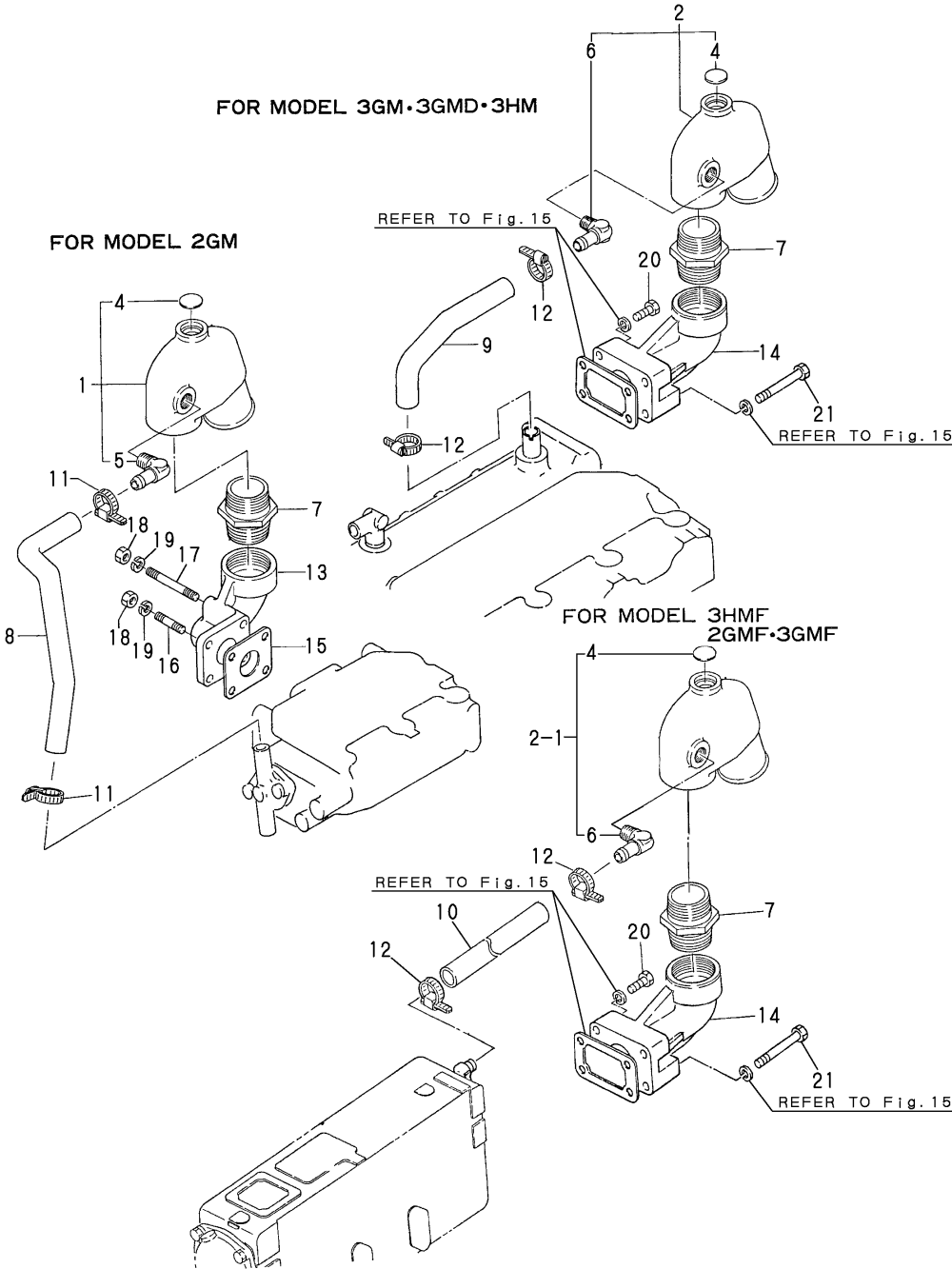
Fig.16.MIXING ELBOW(U-TYPE/OPTIONAL)
