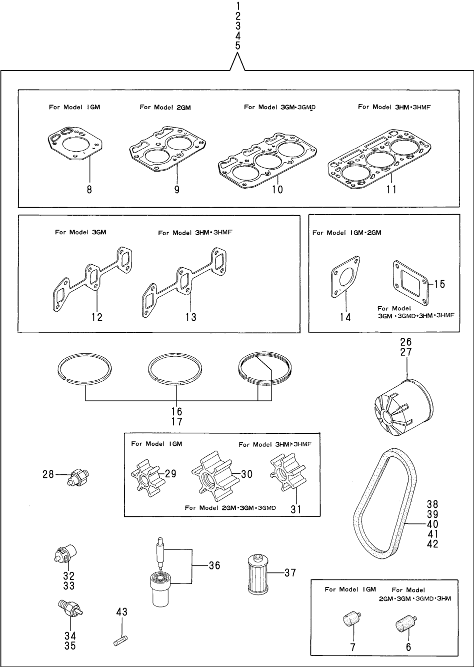
Fig.64.REPAIR KIT(OPTIONAL)
