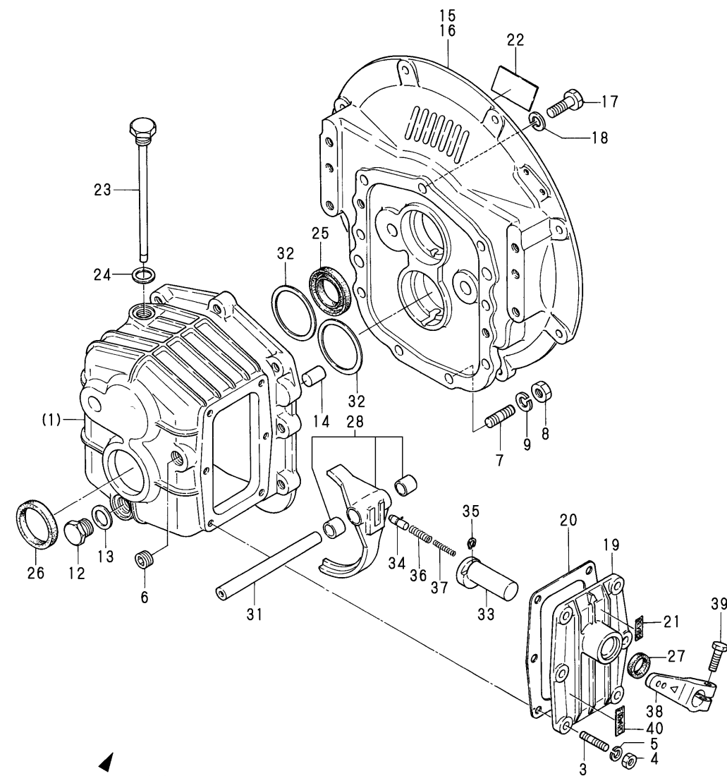
Fig.70.CLUTCH HOUSING
